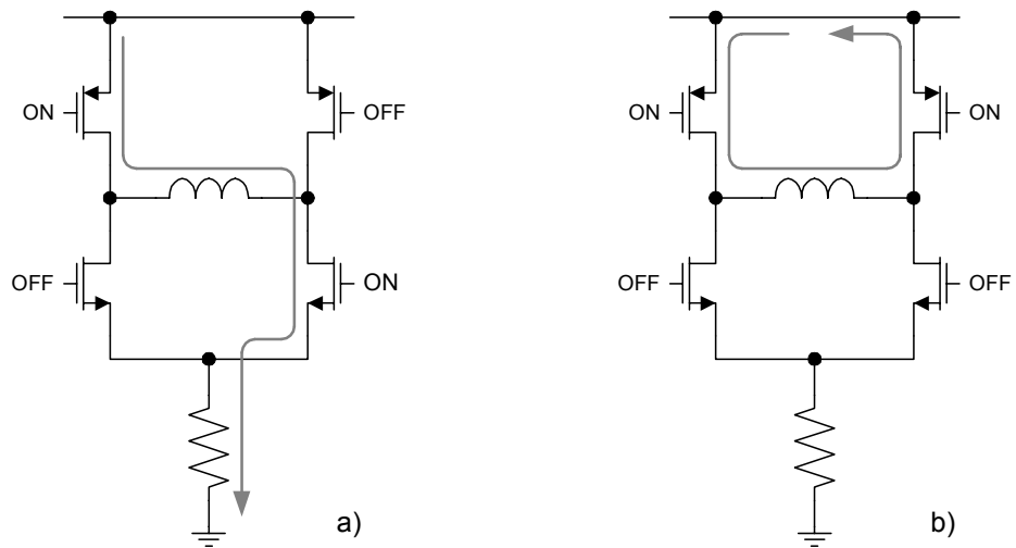
Figure 3-12. Current Flow in Halfbridge
