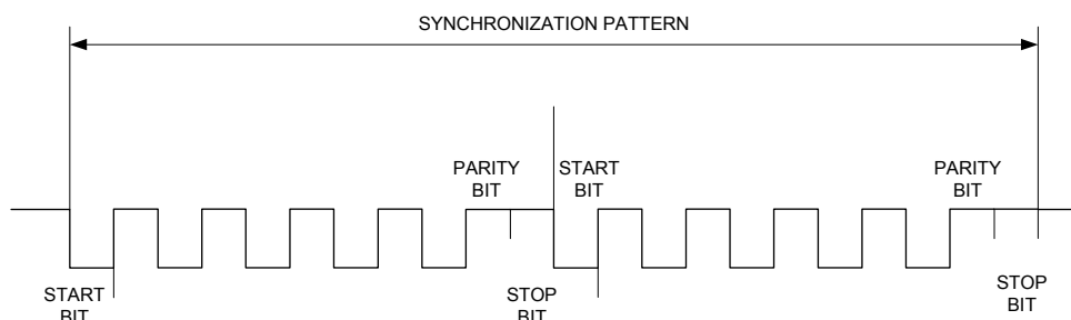
Figure 3-4. Synchronization Sequence
