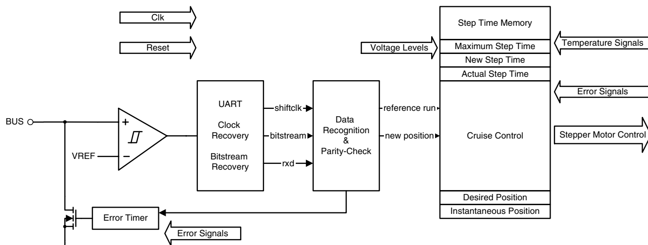
Figure 3-2. Digital Blocks
