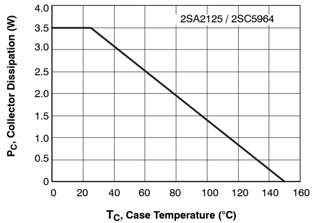
Figure 20. P_C - T_C
