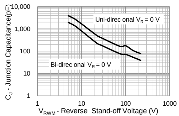
Fig.4 Typical Capacitance
