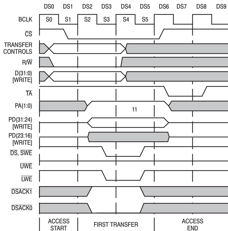
Figure 40. 8-Bit '040 WRITE to 8-Bit Peripheral Example (PA1,PA0=11)
