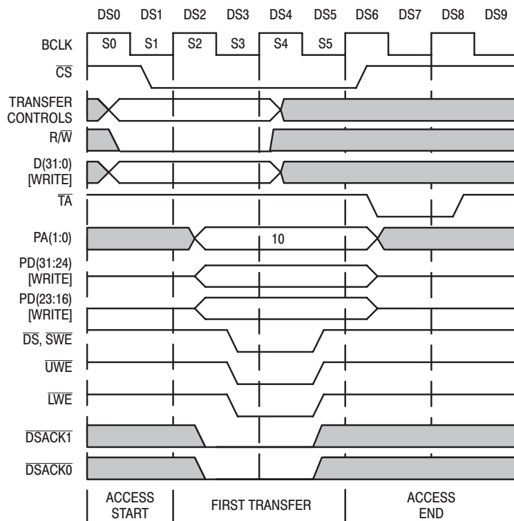
Figure 32. 16-Bit '040 WRITE to 32-Bit Peripheral Example (PA1=1)
