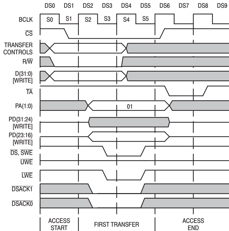
Figure 52. 8-Bit '040 WRITE to 32-Bit Peripheral Example (PA1,PA0=01)
