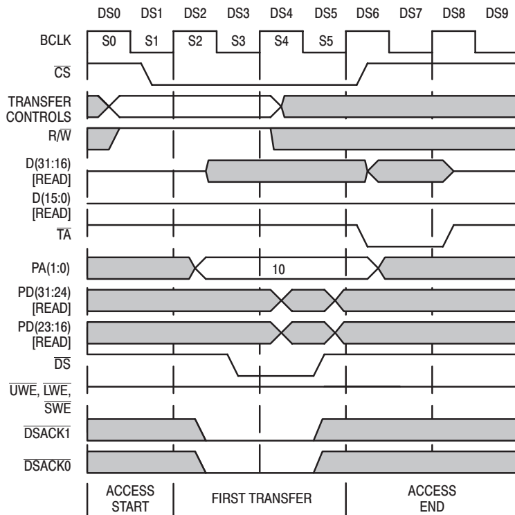
Figure 31. 16-Bit '040 READ From 32-Bit Peripheral Example (PA1=1)
