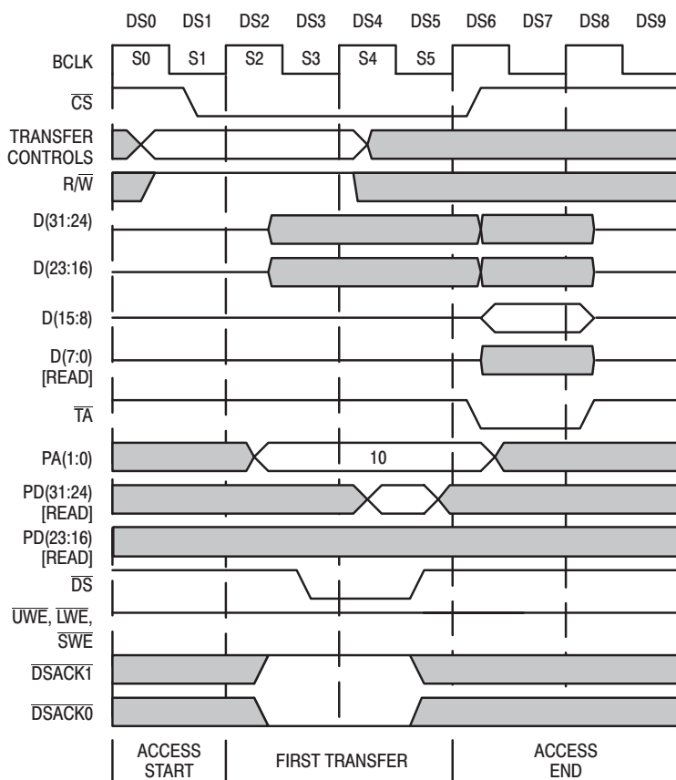
Figure 37. 8-Bit '040 READ From 8-Bit Peripheral Example (PA1,PA0=10)
