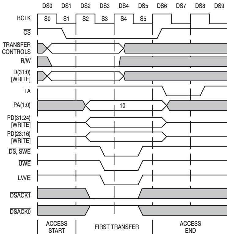
Figure 28. 16-Bit '040 WRITE to 16-Bit Peripheral Example (PA1=1)
