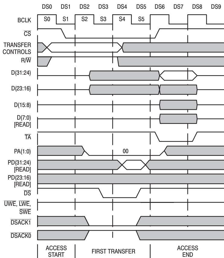
Figure 41. 8-Bit '040 READ From 16-Bit Peripheral Example (PA1,PA0=00)
