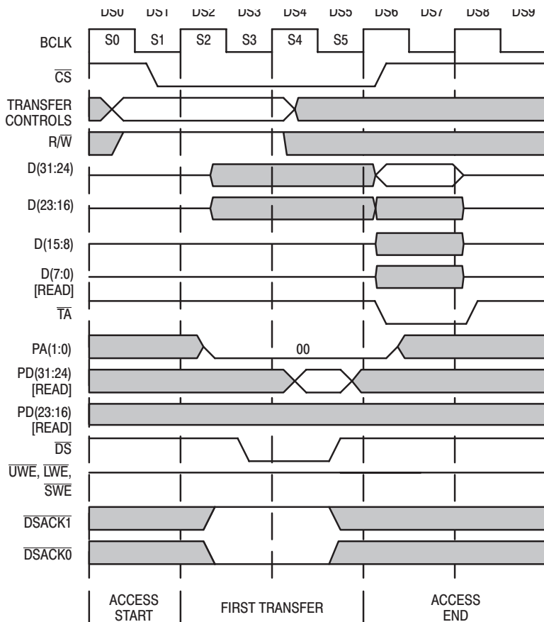
Figure 33. 8-Bit '040 READ From 8-Bit Peripheral Example (PA1,PA0=00)
