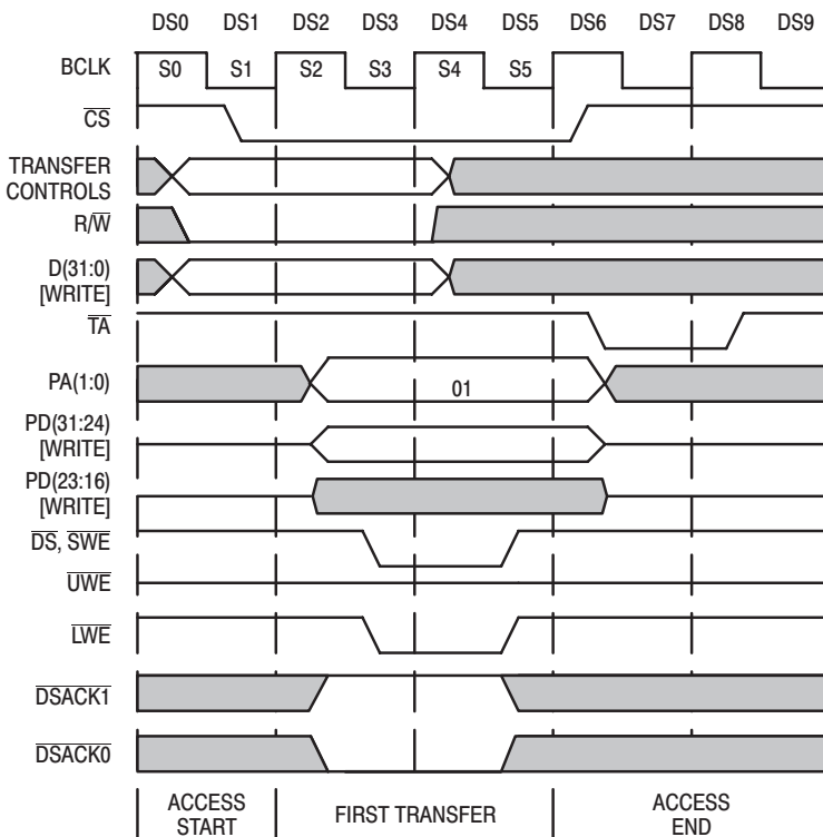
Figure 36. 8-Bit '040 WRITE to 8-Bit Peripheral Example (PA1,PA0=01)
