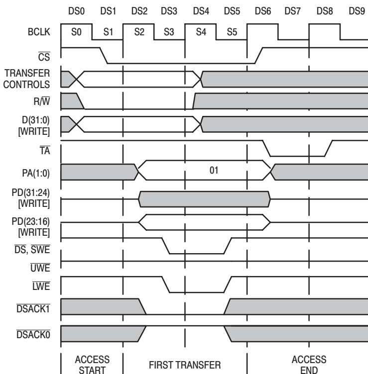
Figure 44. 8-Bit '040 WRITE to 16-Bit Peripheral Example (PA1,PA0=01)
