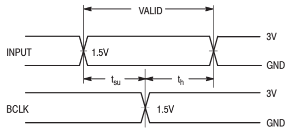
Figure 11. Setup/Hold Times
