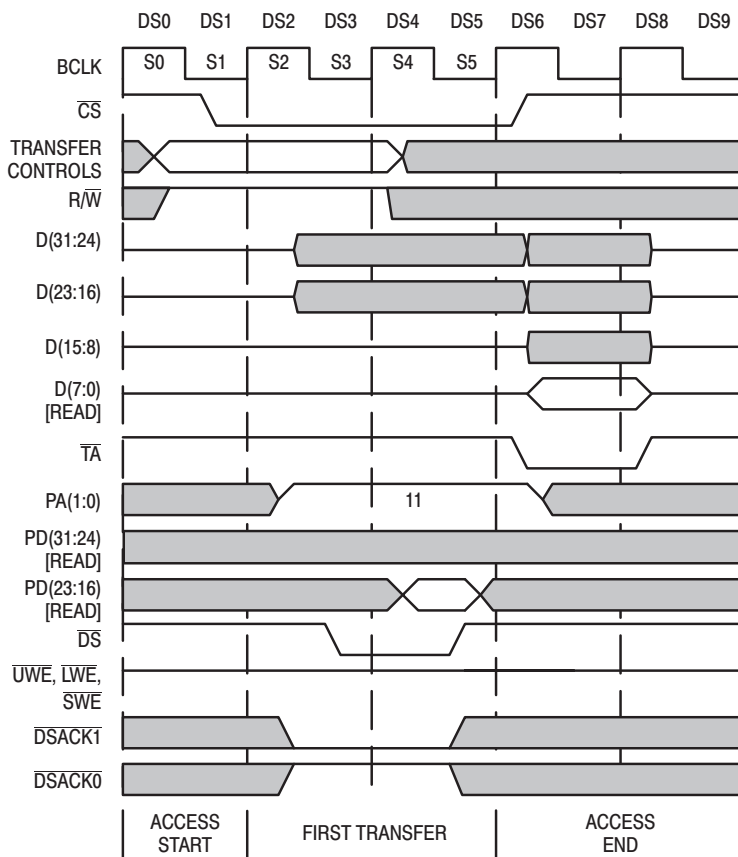
Figure 47. 8-Bit '040 READ From 16-Bit Peripheral Example (PA1,PA0=11)
