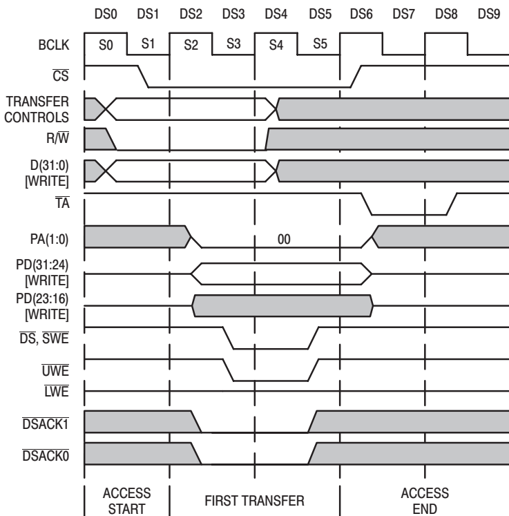
Figure 50. 8-Bit '040 WRITE to 32-Bit Peripheral Example (PA1,PA0=00)
