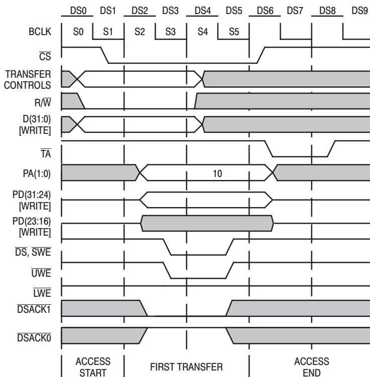
Figure 46. 8-Bit '040 WRITE to 16-Bit Peripheral Example (PA1,PA0=10)
