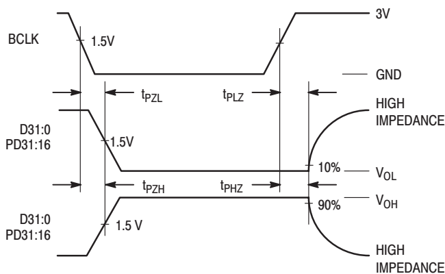
Figure 10. Enable/Disable Times
