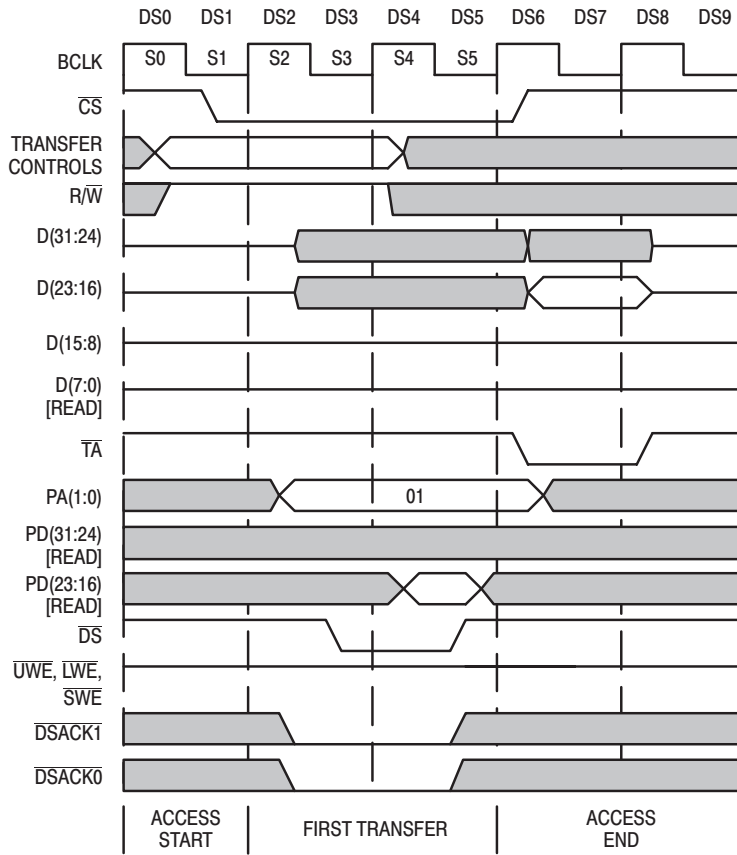
Figure 51. 8-Bit '040 READ From 32-Bit Peripheral Example (PA1,PA0=01)
