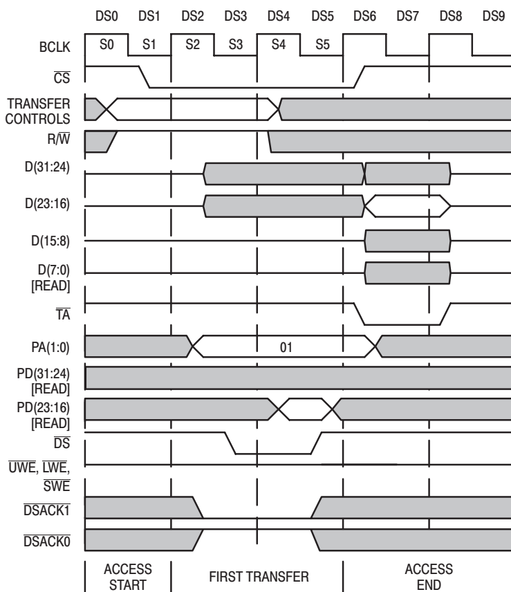
Figure 43. 8-Bit '040 READ From 16-Bit Peripheral Example (PA1,PA0=01)
