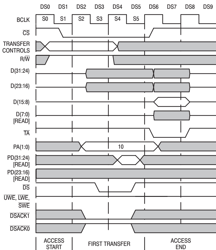
Figure 45. 8-Bit '040 READ From 16-Bit Peripheral Example (PA1,PA0=10)
