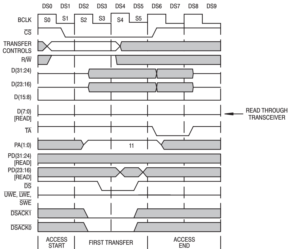
Figure 55. 8-Bit '040 READ From 32-Bit Peripheral Example (PA1,PA0=11)
