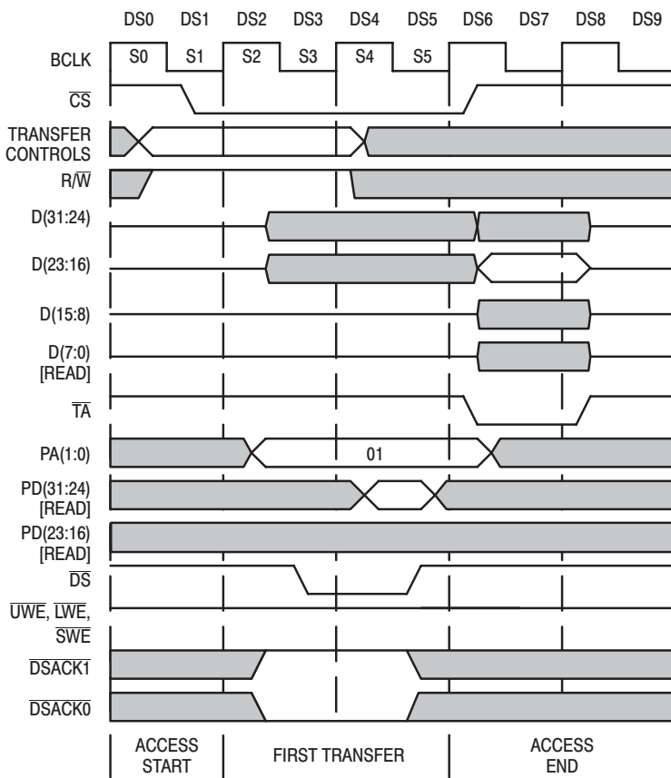
Figure 35. 8-Bit '040 READ From 8-Bit Peripheral Example (PA1,PA0=01)
