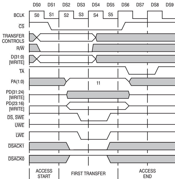
Figure 48. 8-Bit '040 WRITE to 16-Bit Peripheral Example (PA1,PA0=11)
