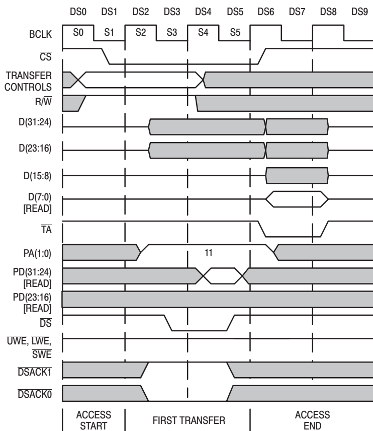
Figure 39. 8-Bit '040 READ From 8-Bit Peripheral Example (PA1,PA0=11)
