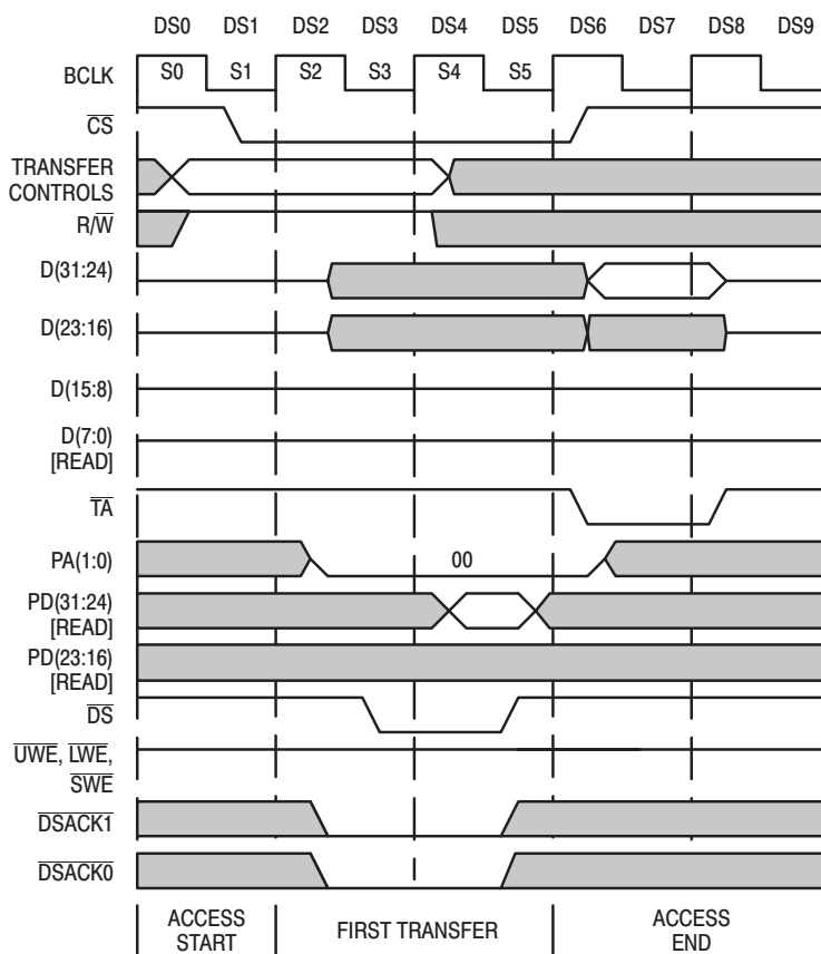
Figure 49. 8-Bit '040 READ From 32-Bit Peripheral Example (PA1,PA0=00)
