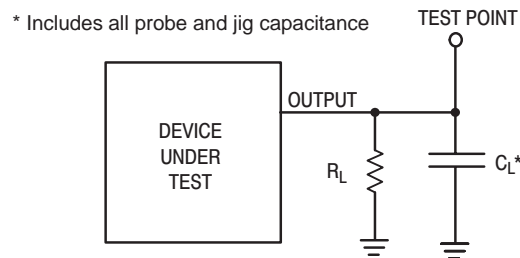
Figure 12. Test Circuit
