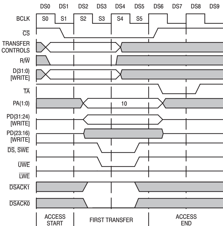
Figure 38. 8-Bit '040 WRITE to 8-Bit Peripheral Example (PA1,PA0=10)
