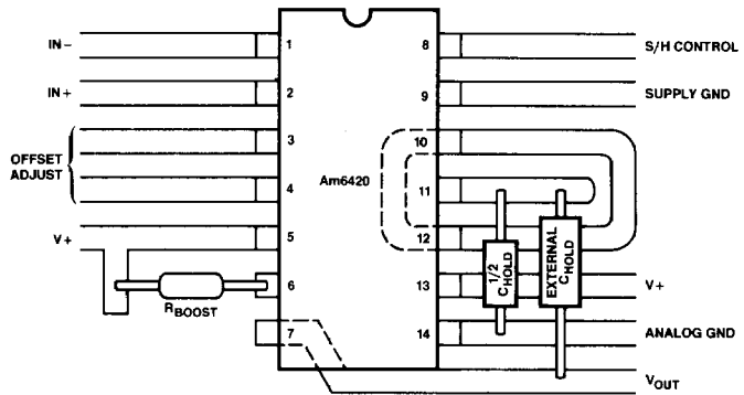
Figure 8. Pad Layout – Top View
