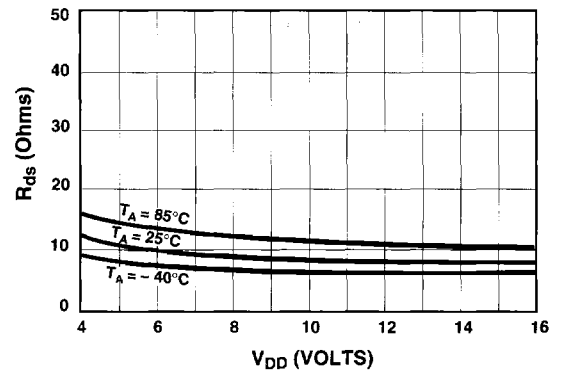
Low-State Output Resistance
