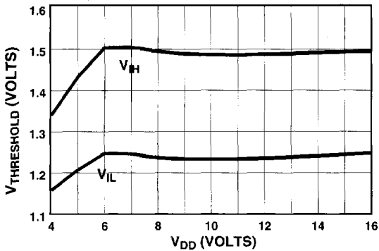
Input Threshold vs. Supply Voltage T_A = 25^\circ\text{C}
