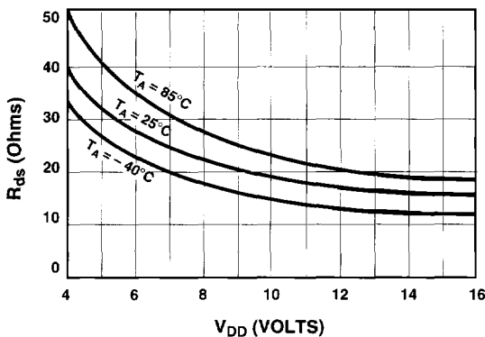
High-State Output Resistance
