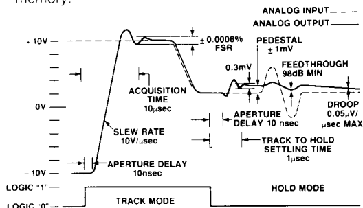
Figure 2. Pictorial Showing Various S/H Characteristics
