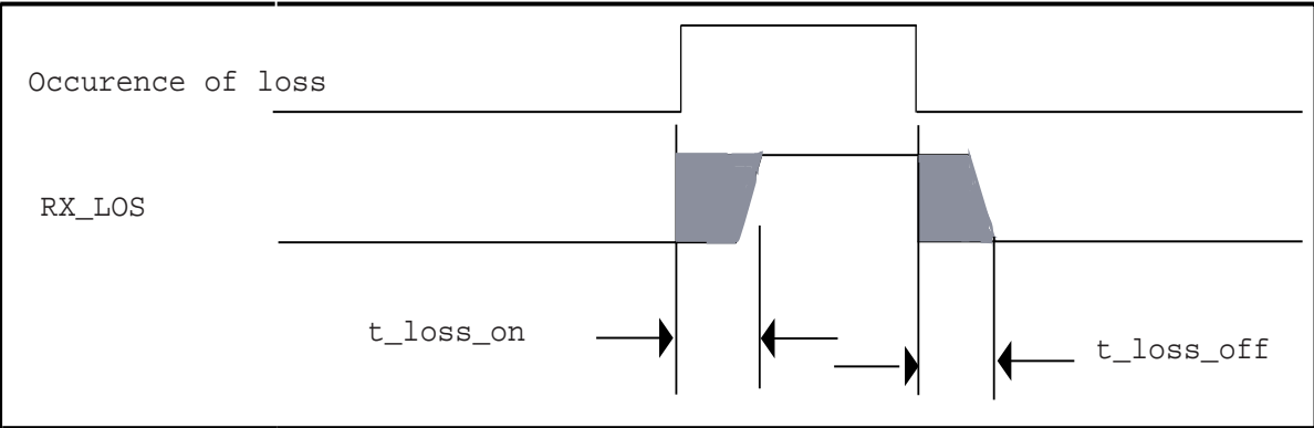
Figure 10: Timing of RX_LOS detection
