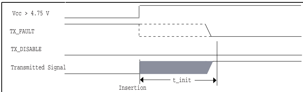
Figure 5: Example of initialization during hot plugging with TX_DISABLE negated.
