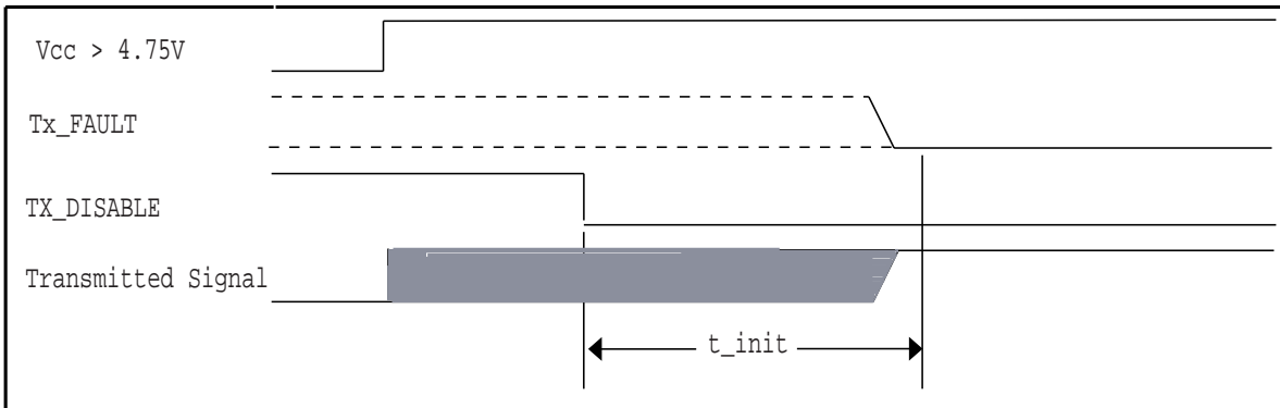
Figure 4: Power on initialization of GBIC with TX_DISABLE asserted
