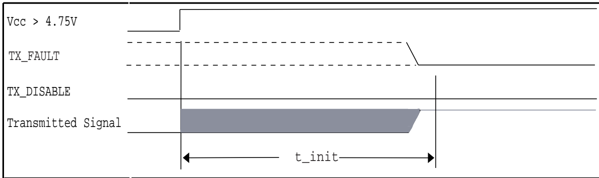
Figure 3: Power on initialization of GBIC with TX_DISABLE negated
