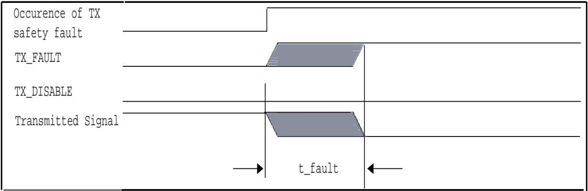
Figure 7: Detection of transmitter safety fault condition
