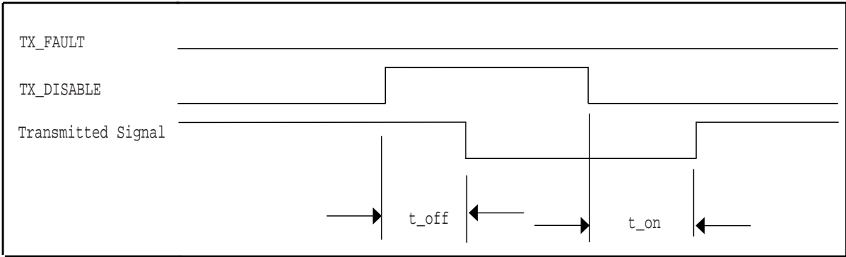
Figure 6: Management of GBIC during normal operation with TX_DISABLE implemented.
