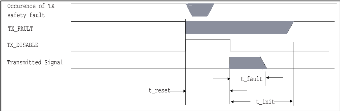
Figure 9: Unsuccessful recovery from safety fault condition
