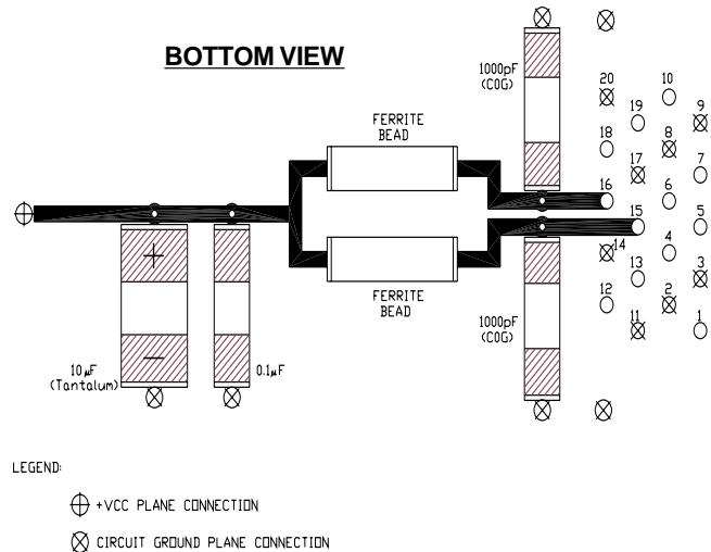
Figure 2B. Suggested Power Coupling
