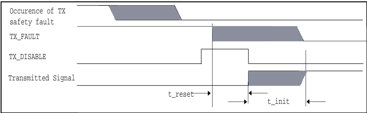
Figure 8: Successful recovery from transient safety fault condition
