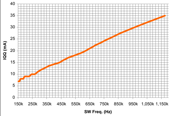
IQQ VS. FREQUENCY
