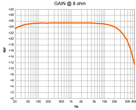
GAIN @ 8 OHM
