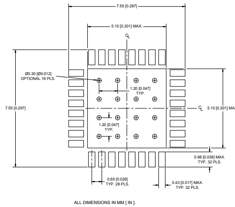
Figure 5 – Recommended Land Pad with Vias for 7x7mm LQ package
