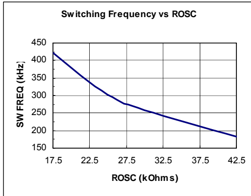
Figure 4 – Typical Switching Frequency vs. ROSC
