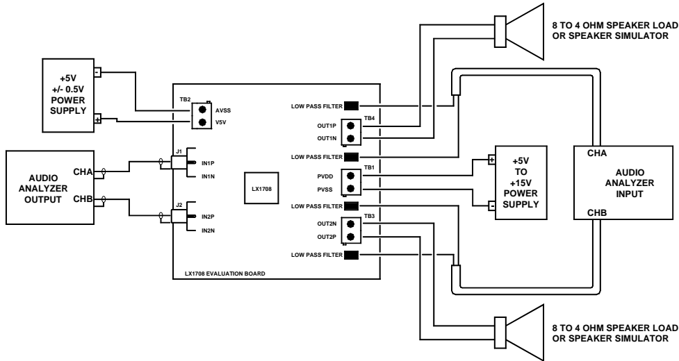
Figure 2 – System Test Set-up Diagram
