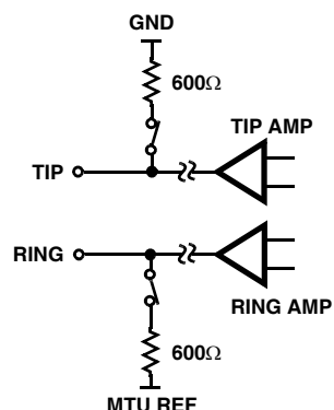
FIGURE 8. LPS 2-WIRE INTERFACE CIRCUIT DIAGRAM
