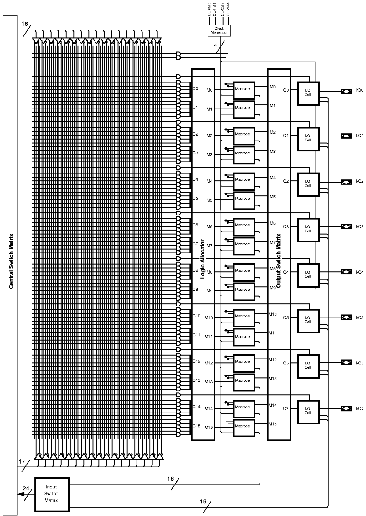
Figure 1. M4-128N (M4LV-128N) PAL Block
