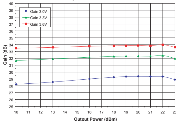
Figure 6: Gain vs. Output Power Across Power Supply Voltage (Frequency = 2.45GHz, T_c = 25^\circ C ) 802.11g 54 Mbps OFDM
