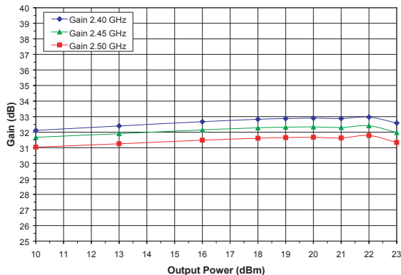
Figure 2: Gain vs. Output Power Across Frequency ( V_{CC} = +3.3V , T_c = +25^\circ C ) 802.11g 54 Mbps OFDM
