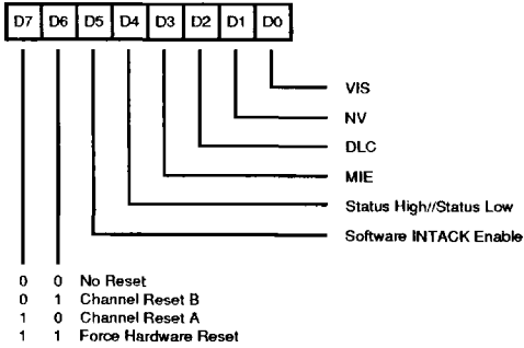
Write Register 9
