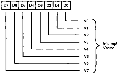
Write Register 2
