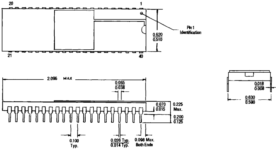
40-Pin Ceramic DIP Package Diagram
