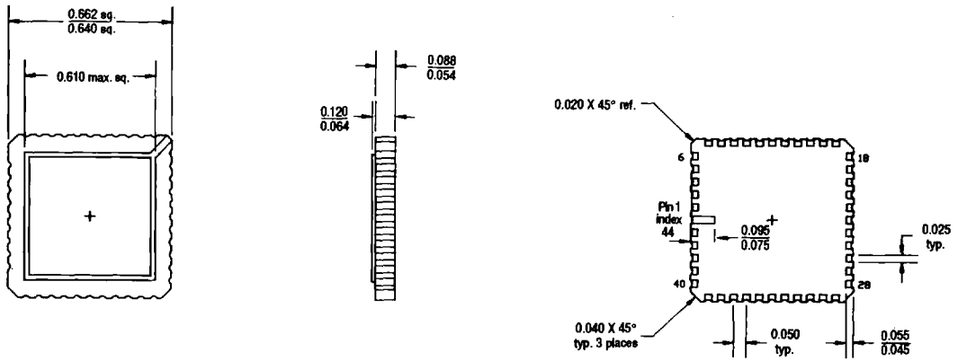
44-Pin Ceramic LCC Package Diagram
