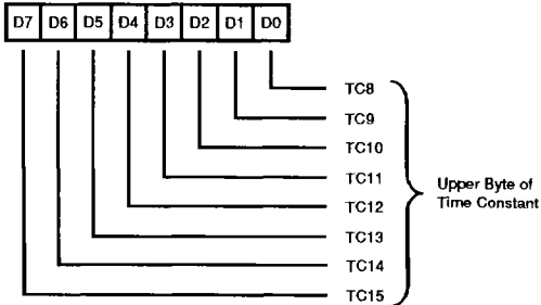
Write Register 13
