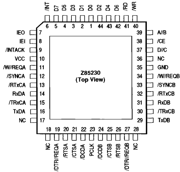
Figure 3. Z85230 LCC Pin Assignments
