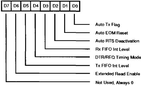
WR 7 Prime
