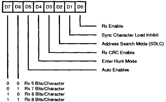
Write Register 3
