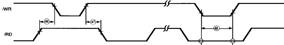
Figure 26. Reset Timing Diagram
