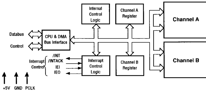
Figure 1. ESCC Block Diagram
