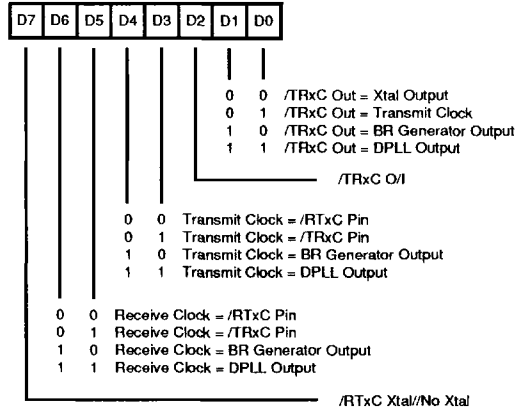
Write Register 11
