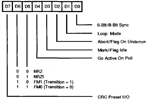
Write Register 10
