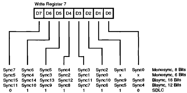
Figure 18. Write Register Bit Functions (Continued)
