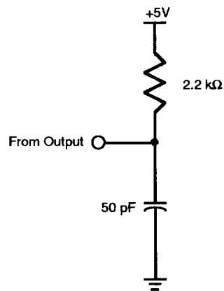
Figure 24. Open-Drain Test Load
