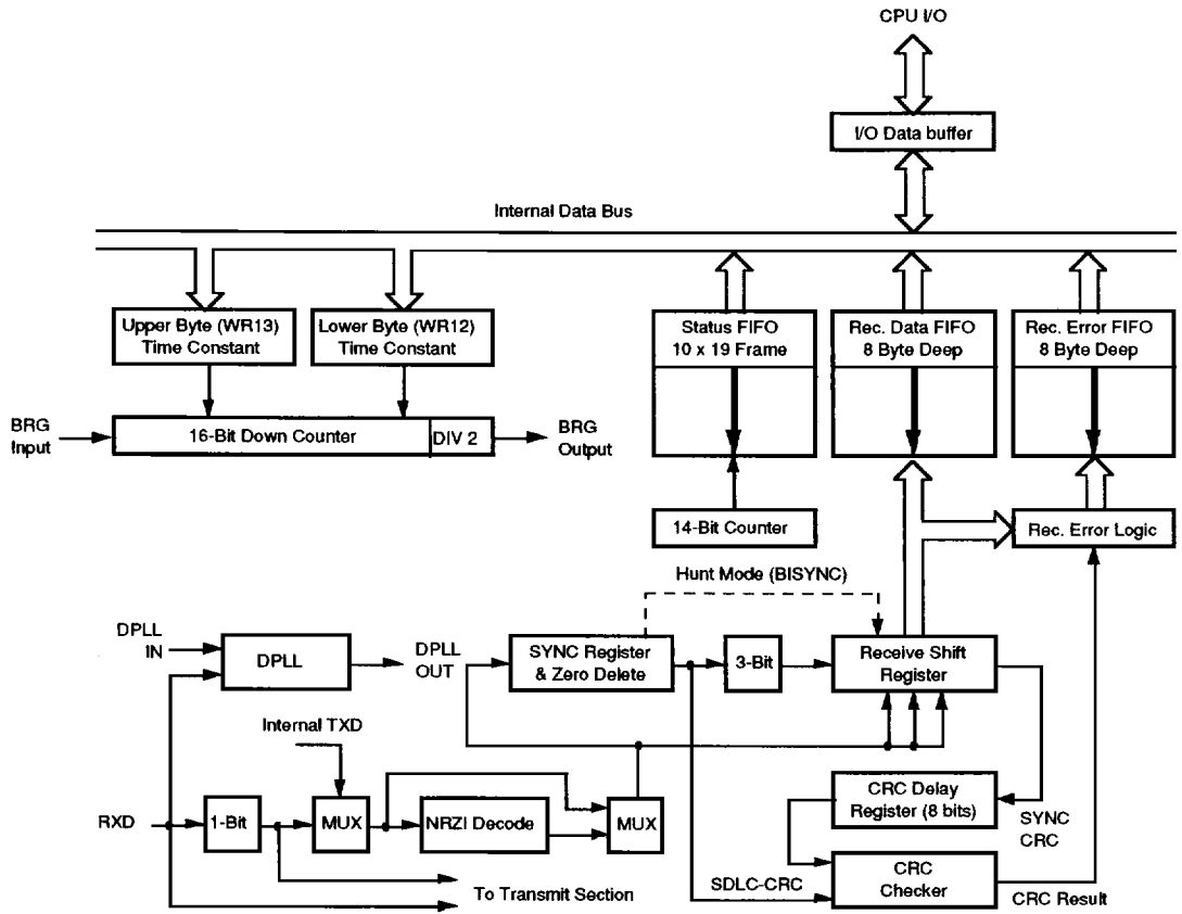
Figure 6. ESCC Receive Data Path
