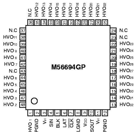
Outline 48P6D-A (GP)
