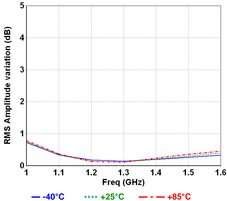
RMS Amplitude Variation versus Frequency
