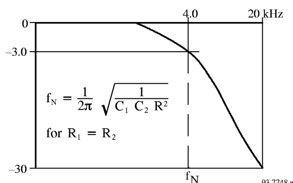
Figure 9. Low-pass filter
