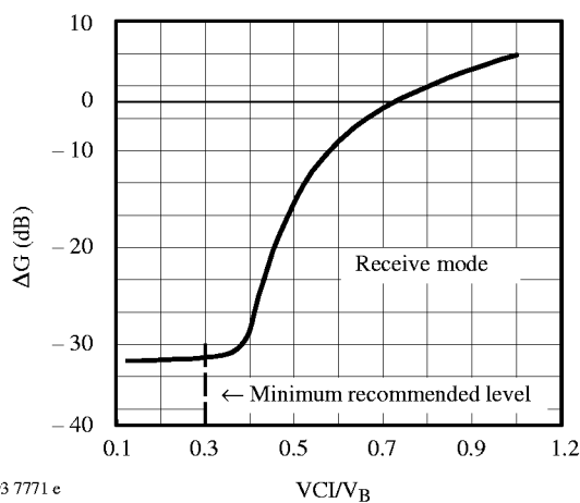
Figure 15. Receive attenuator versus volume control
