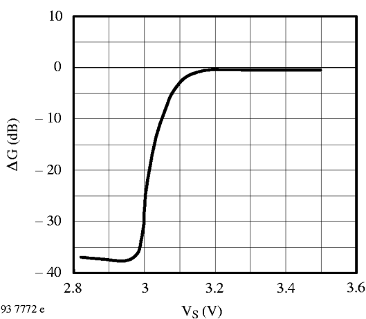
Figure 16. Receive attenuation gain versus VS
