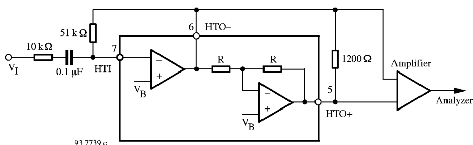
Figure 10. Hybrid amplifier distortion test
