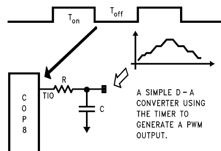
FIGURE 11. Timer Application
