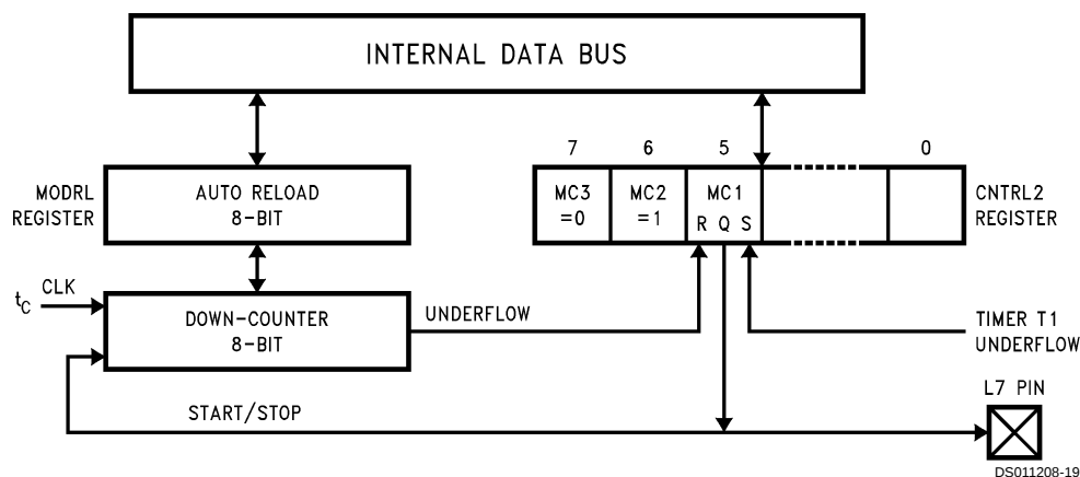
FIGURE 14. Mode 2a: 50% Duty Cycle Output
