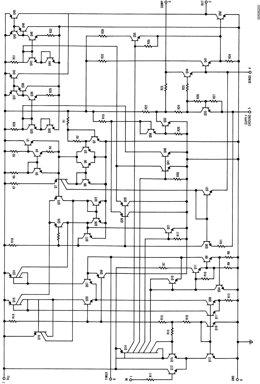
FIGURE 2. LM1949 Circuit
