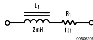
FIGURE 3. Model of a Typical Fuel Injector
