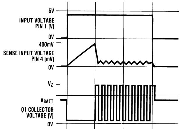
FIGURE 6. Switching Waveforms
