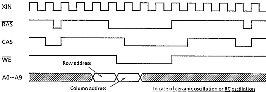
Fig 5.14 Address counter
