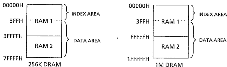
Fig. 5.5 Configuration of index area and data area
