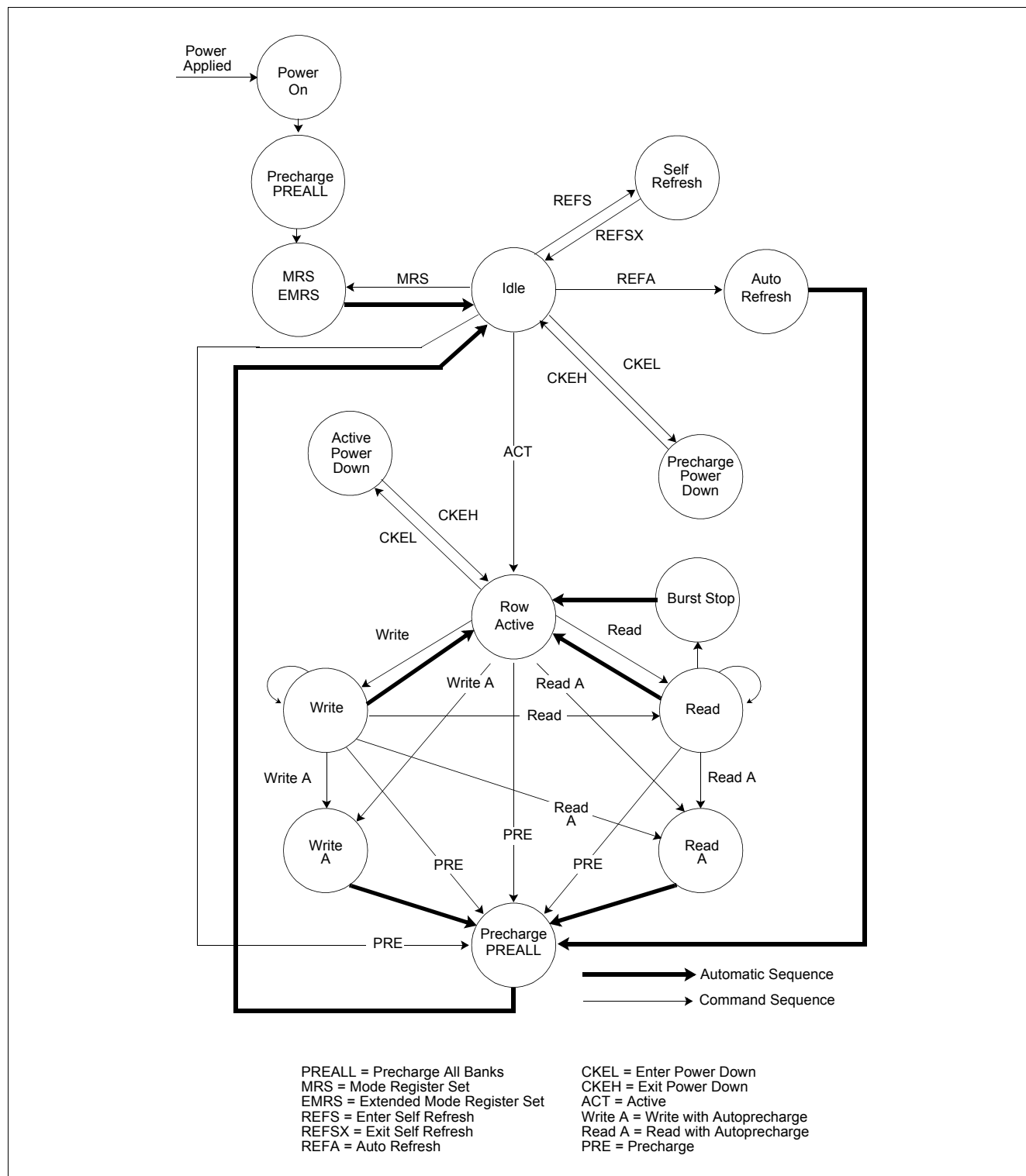
Figure 33 Simplified State Diagram
