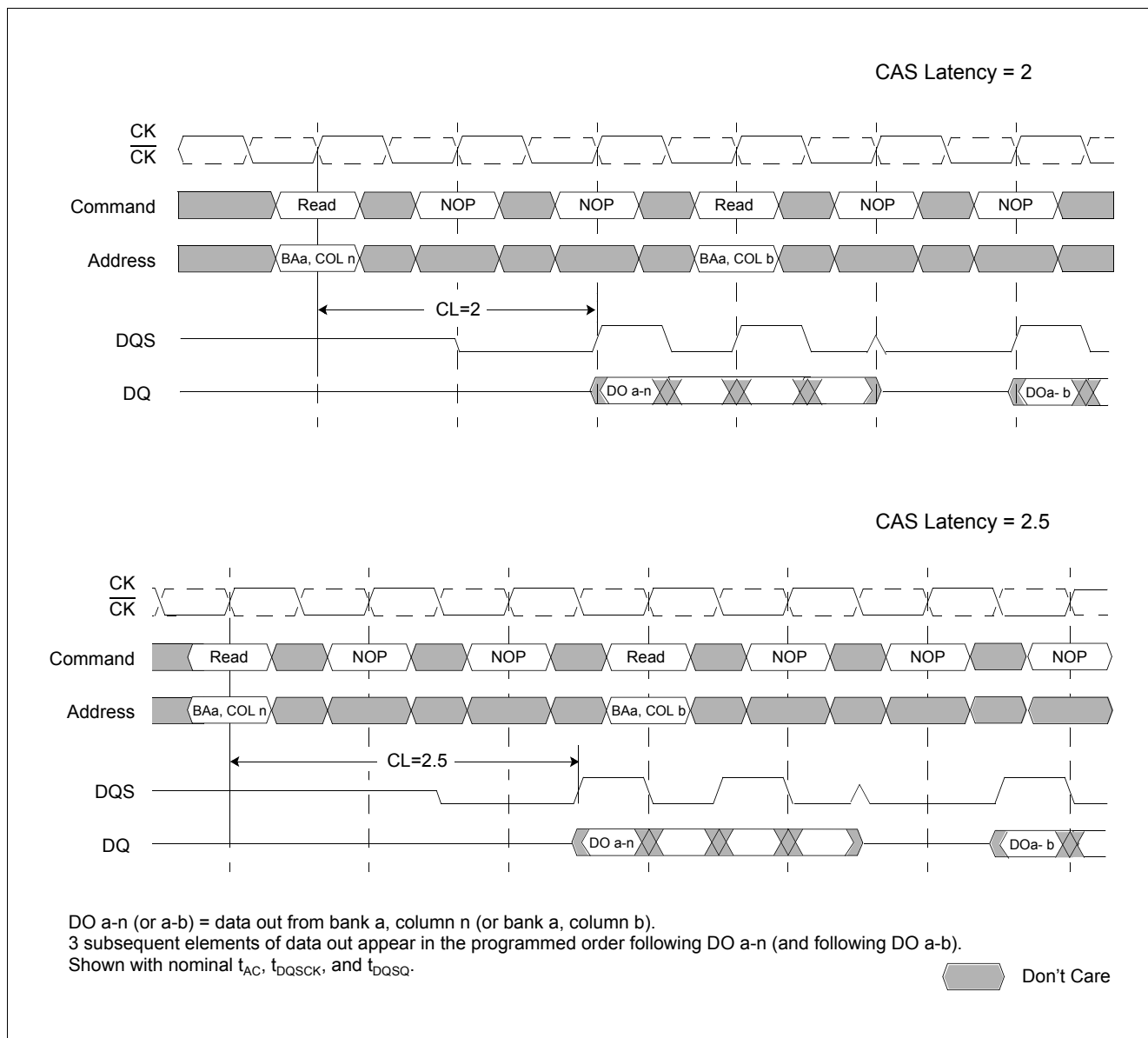
Figure 12 Non-Consecutive Read Bursts: CAS Latencies (Burst Length = 4)
