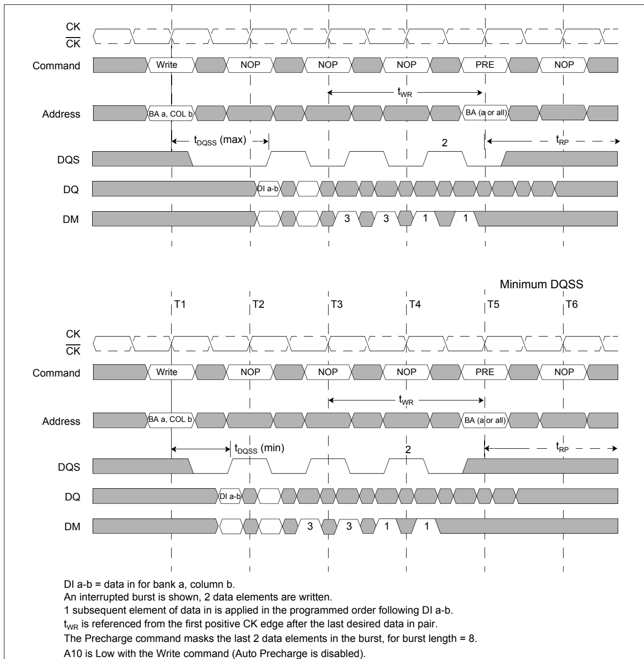
Figure 27 Write to Precharge: Interrupting (Burst Length = 4 or 8)
