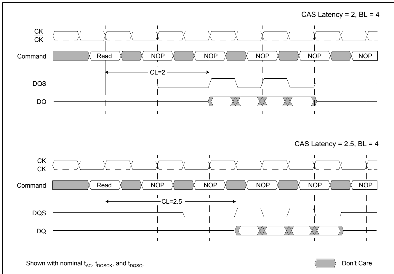
Figure 6 Required CAS Latencies
