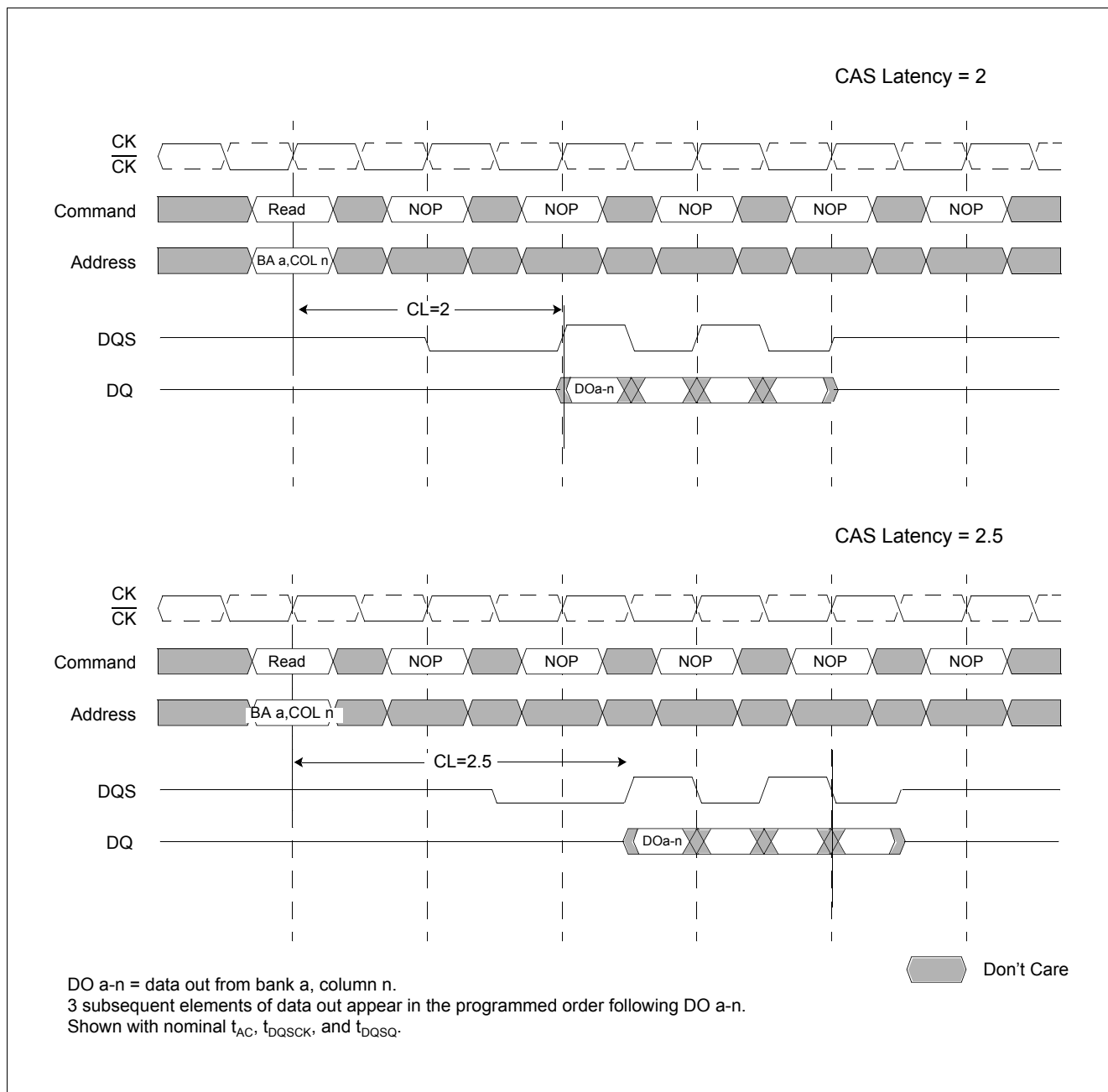
Figure 10 Read Burst: CAS Latencies (Burst Length = 4)
