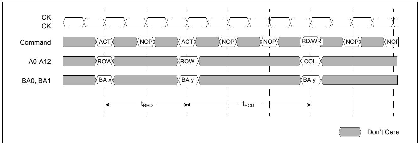
Figure 8 t_{RCD} and t_{RRD} Definition
