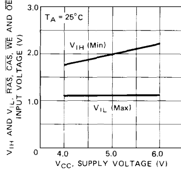
Fig. 18 – RAS, CAS, WE AND OE INPUT VOLTAGE vs. SUPPLY VOLTAGE
