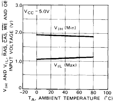
Fig. 19 – RAS, CAS, WE AND OE INPUT VOLTAGE vs. AMBIENT TEMPERATURE
