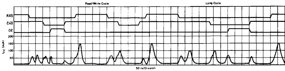
Fig. 2 – CURRENT WAVEFORM ( V_{CC} = 5.5\text{ V} , T_A = 25^\circ\text{C} )
