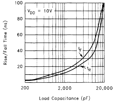
Rise/Fall Time vs Load
