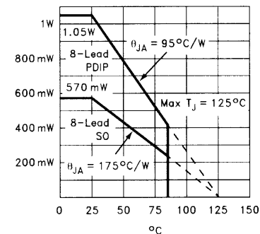
Max Power/Derating Curves
