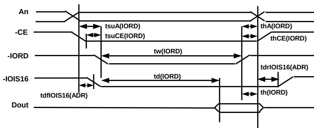
True IDE Mode Access Read Timing
