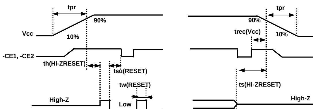
Hard Reset Timing
