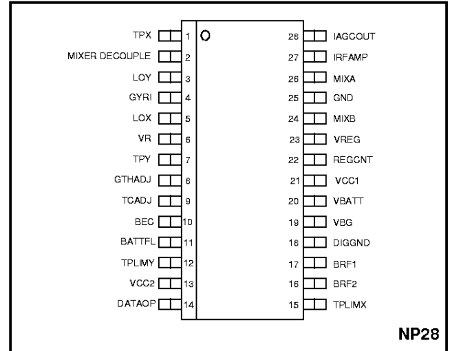
Fig.1 Pin connections
