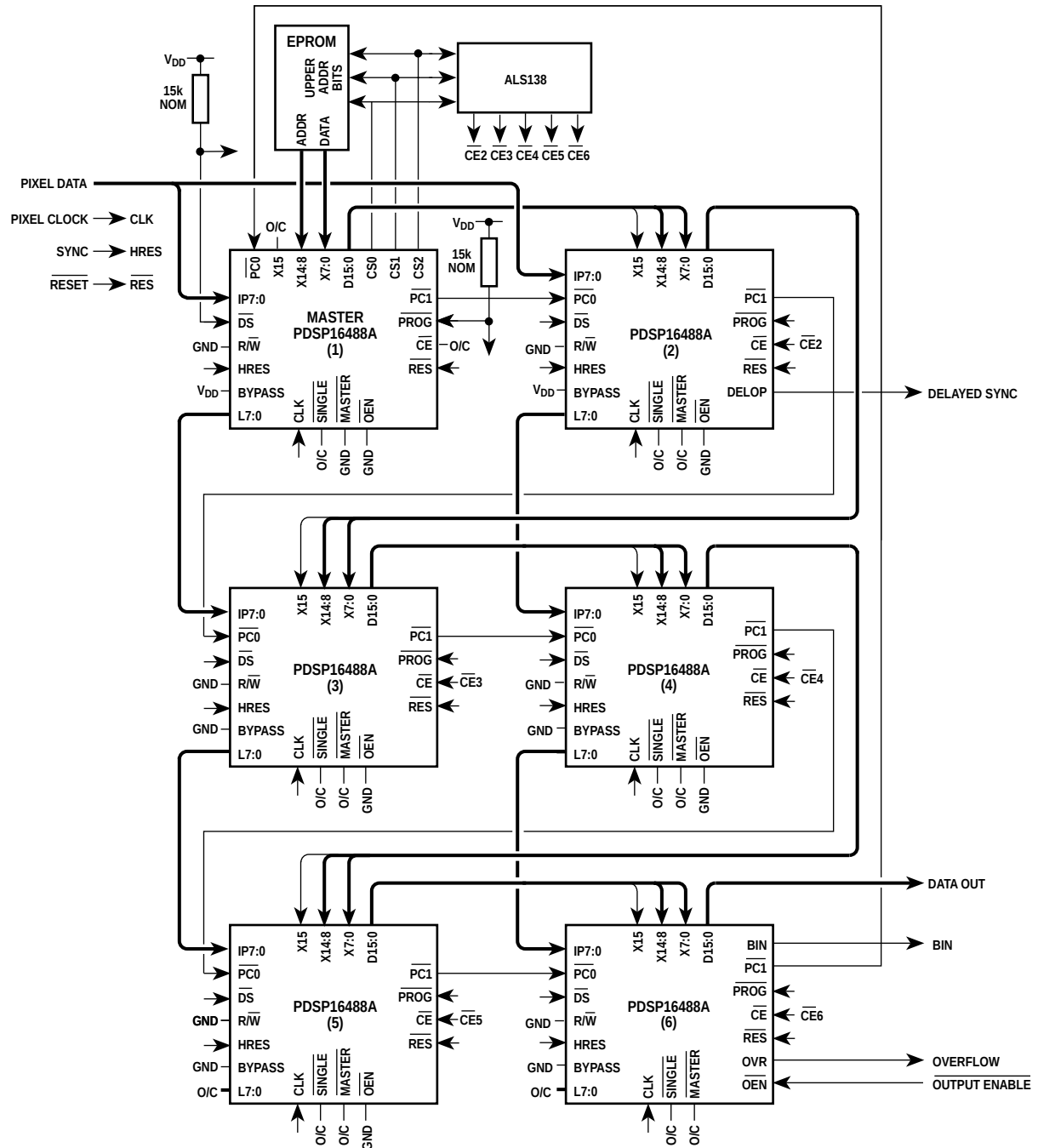
Fig. 19 Six device non-interlaced system.
