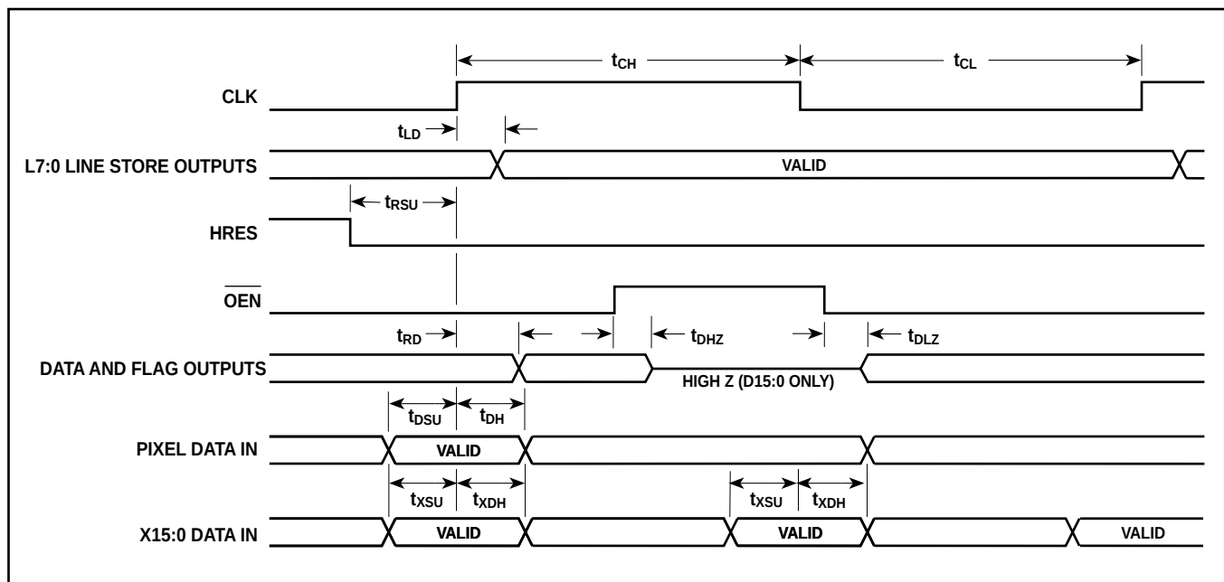
Fig. 12 Operational timing
