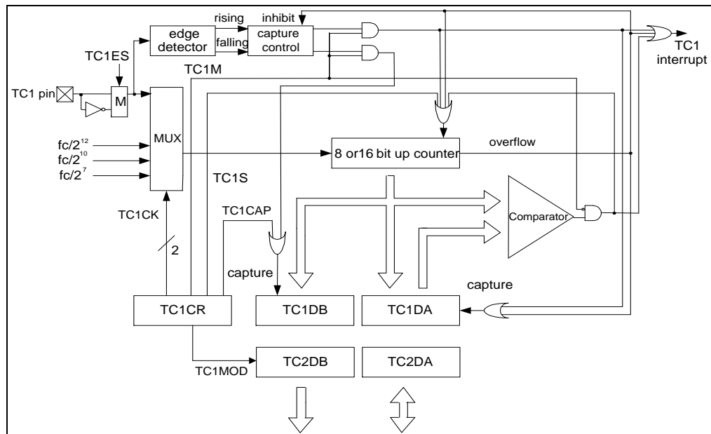
Figure 6-17 Timer / Counter 1 Configuration
