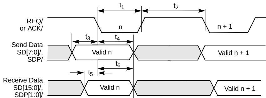
Figure 6.42 Initiator and Target Synchronous Transfers
