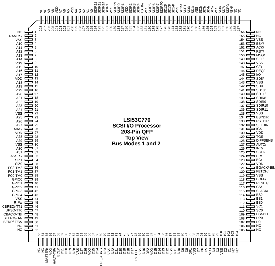
Figure 3.1 LSI53C770 Pin Diagram, Bus Modes 1 and 2
