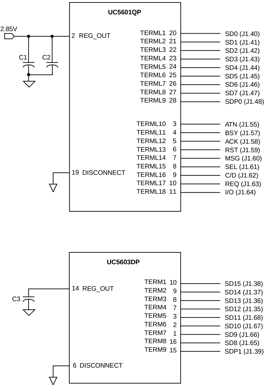
Figure 2.7 Regulated Termination
