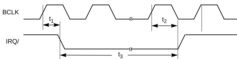
Figure 6.8 Interrupt Output Waveforms
