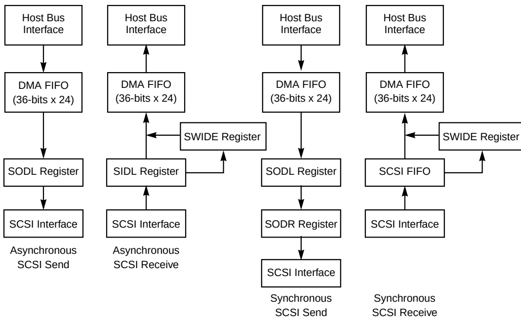
Figure 2.2 LSI53C770 Data Paths
