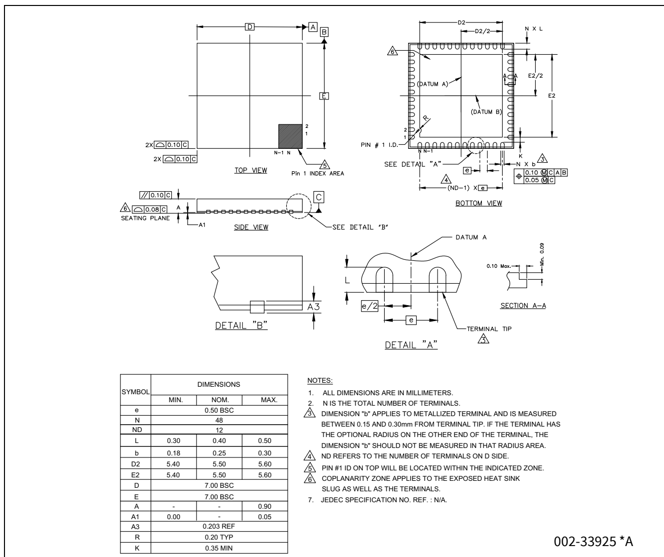
Figure 8 48-pin QFN (7 × 7 × 0.9 mm) package outline, 002-33925
