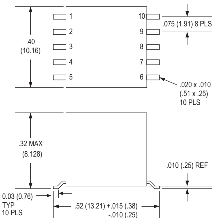
FIGURE 4. MECHANICAL OUTLINE
