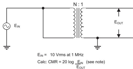
FIGURE 2. CIRCUIT FOR COMMON MODE REJECTION
