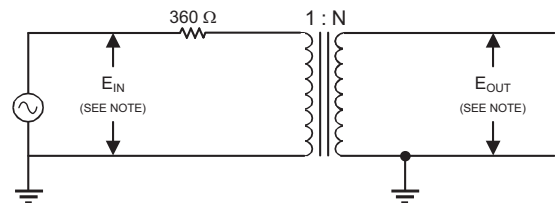
FIGURE 2. CIRCUIT FOR COMMON MODE REJECTION
