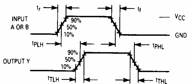
Figure 1 Switching Waveforms.
