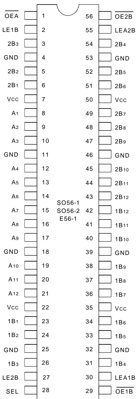
SSOP/ TSSOP/ CERPACK TOP VIEW
