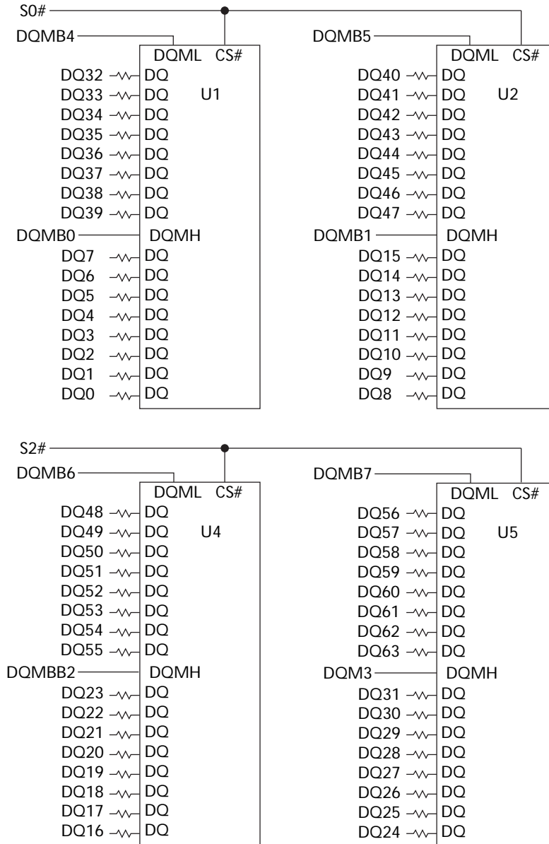
Figure 3: Functional Block Diagram
