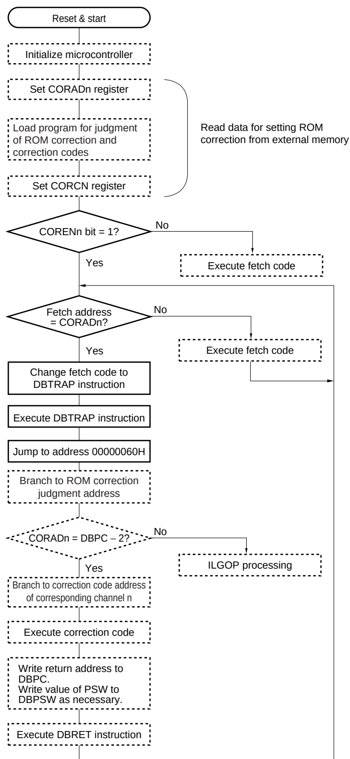
Figure 29-2. ROM Correction Operation and Program Flow
