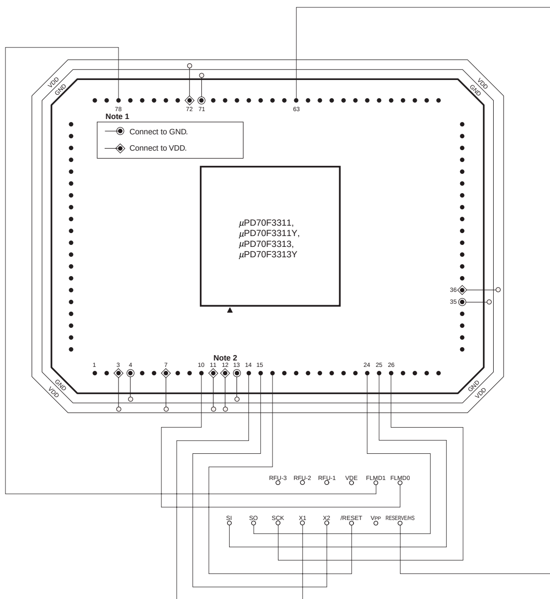
Figure 31-7. Wiring Example of V850ES/KG1+ Flash Writing Adapter (FA-100GF-3BA-A)
