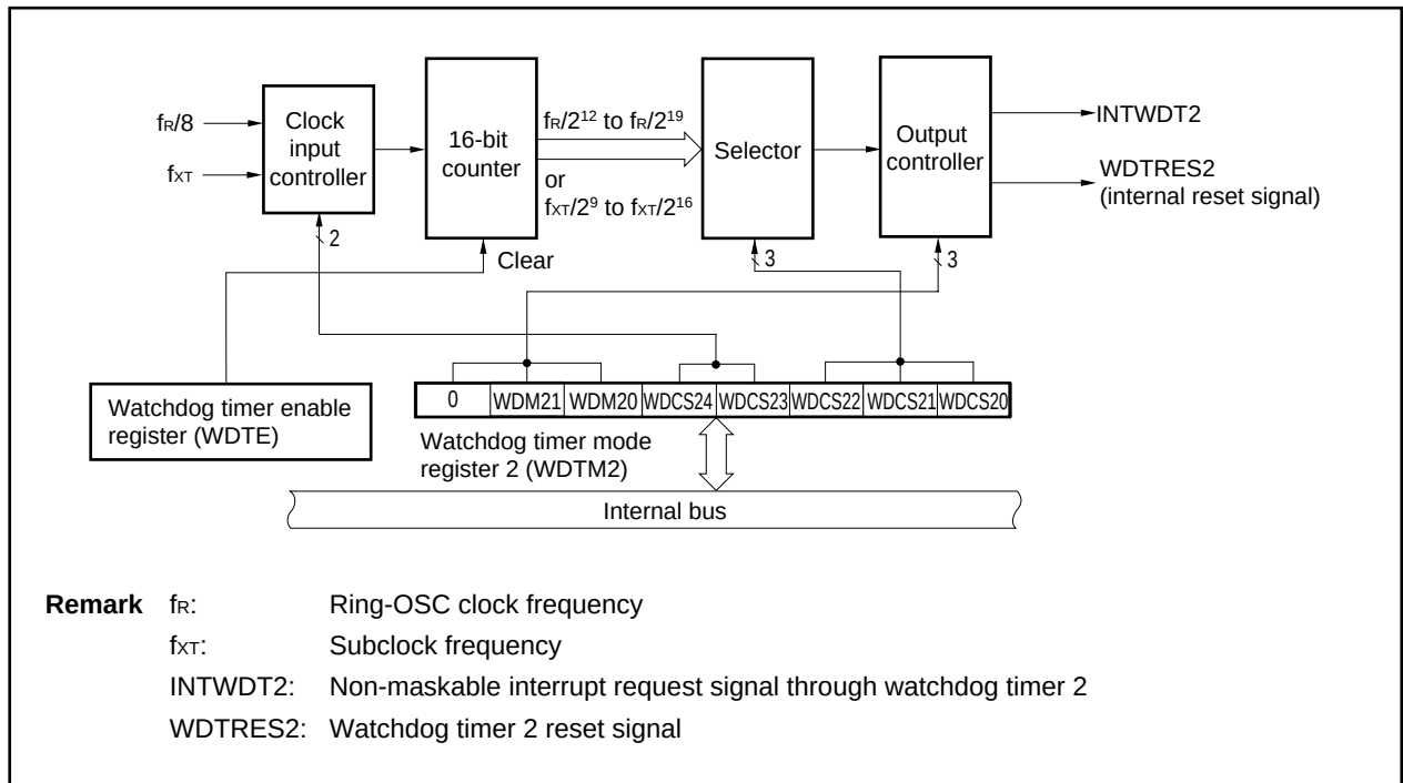
Figure 12-2. Block Diagram of Watchdog Timer 2
