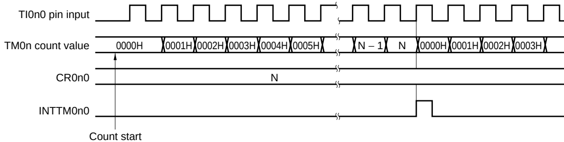
Figure 8-20. Timing of External Event Counter Operation (with Rising Edge Specified)
