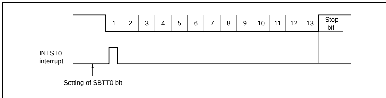
Figure 16-15. SBF Transmission
