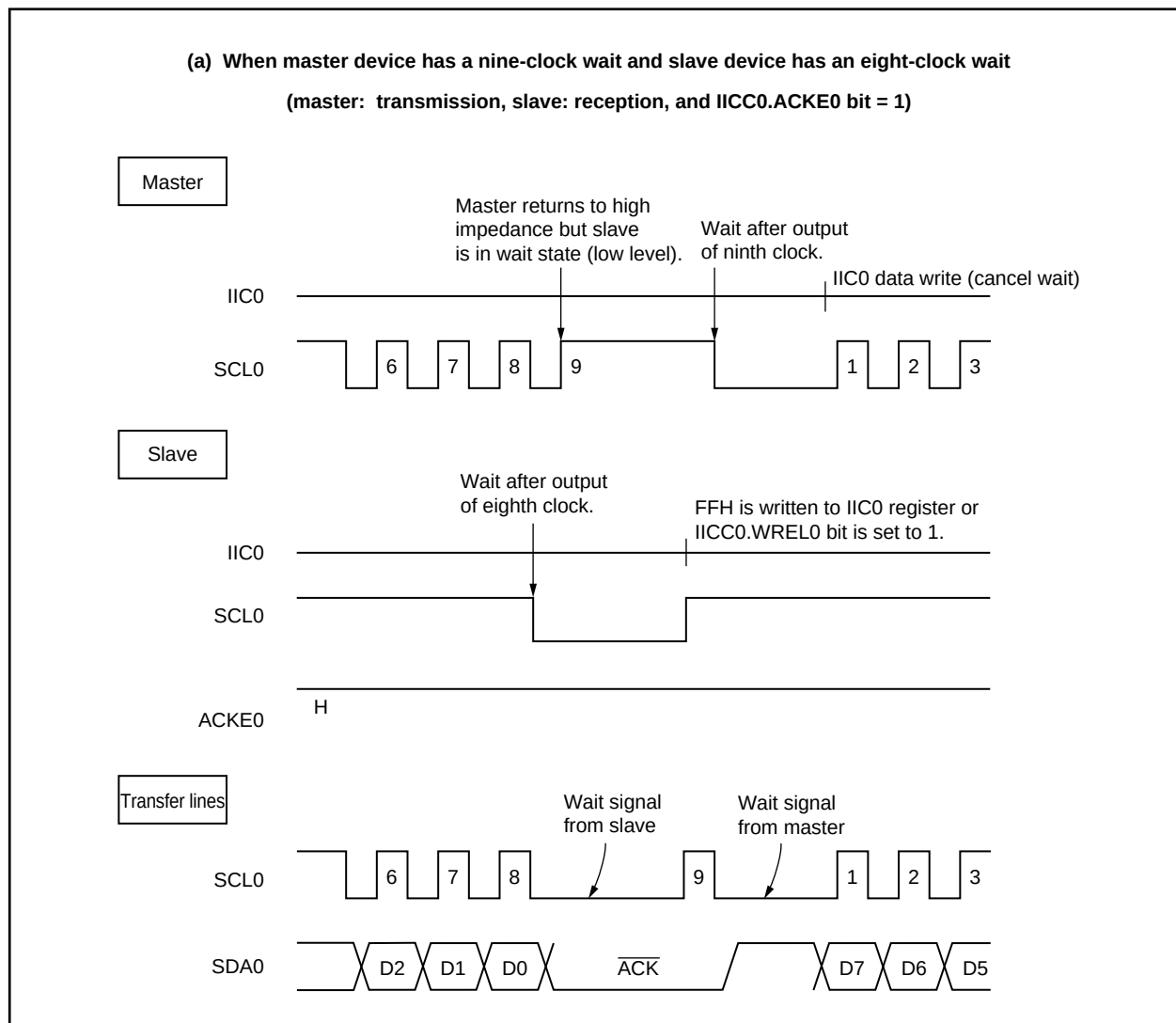
Figure 19-10. Wait Signal (1/2)
