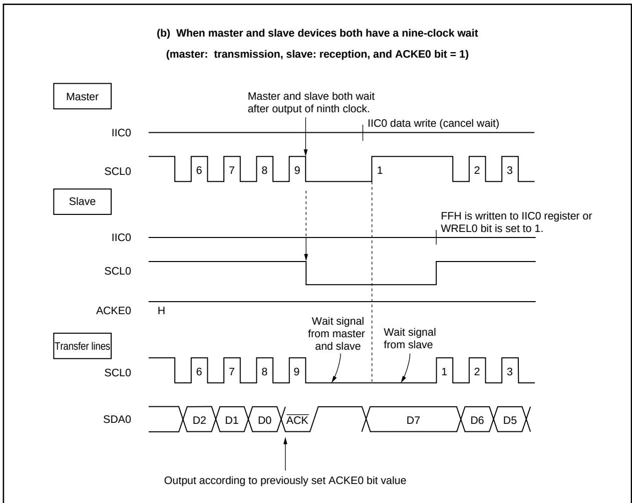
Figure 19-10. Wait Signal (2/2)
