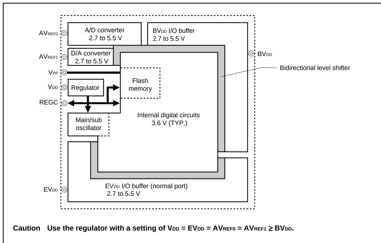
Figure 28-1. Regulator
