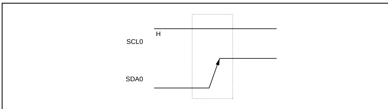
Figure 19-9. Stop Condition
