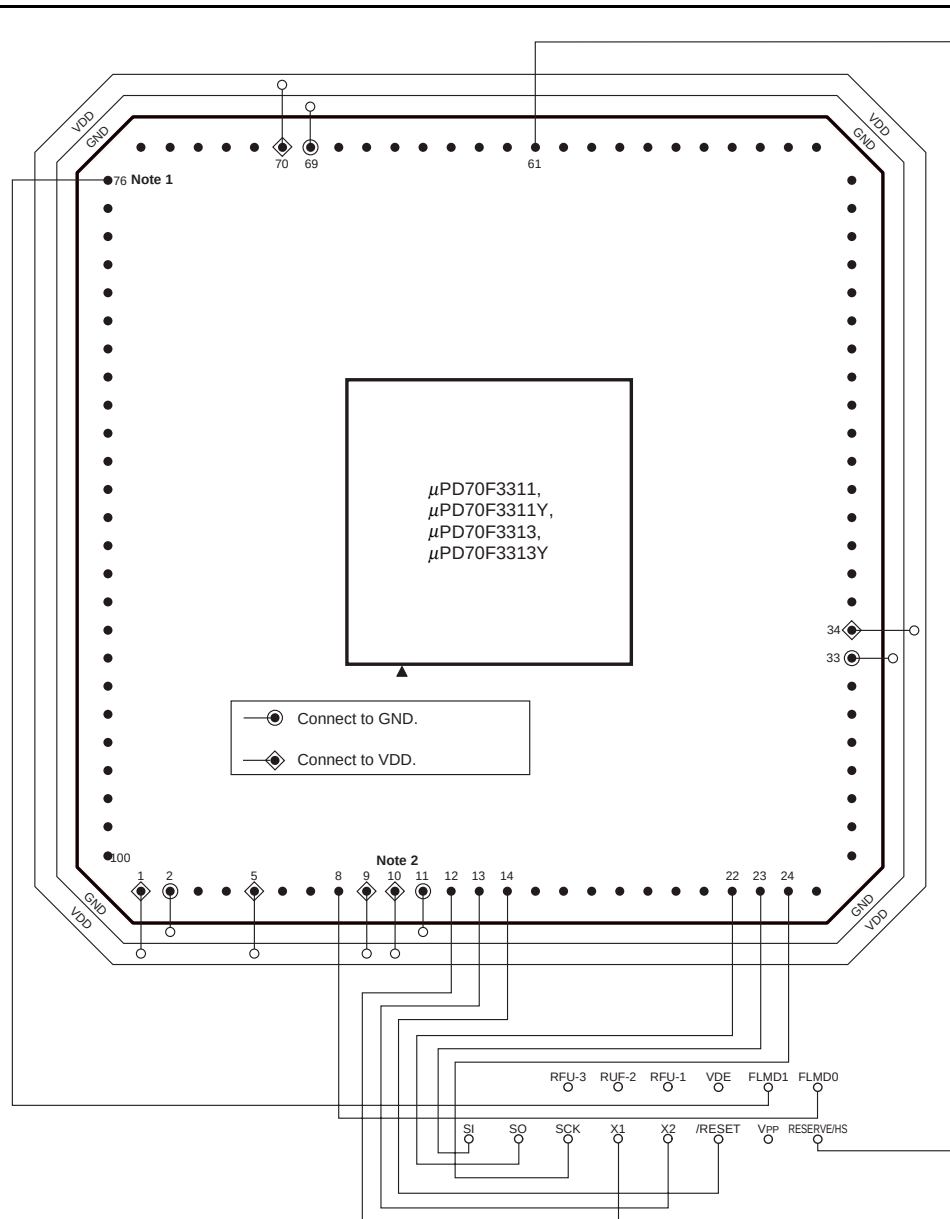
Figure 31-6. Wiring Example of V850ES/KG1+ Flash Writing Adapter (FA-100GC-8EU-A)
