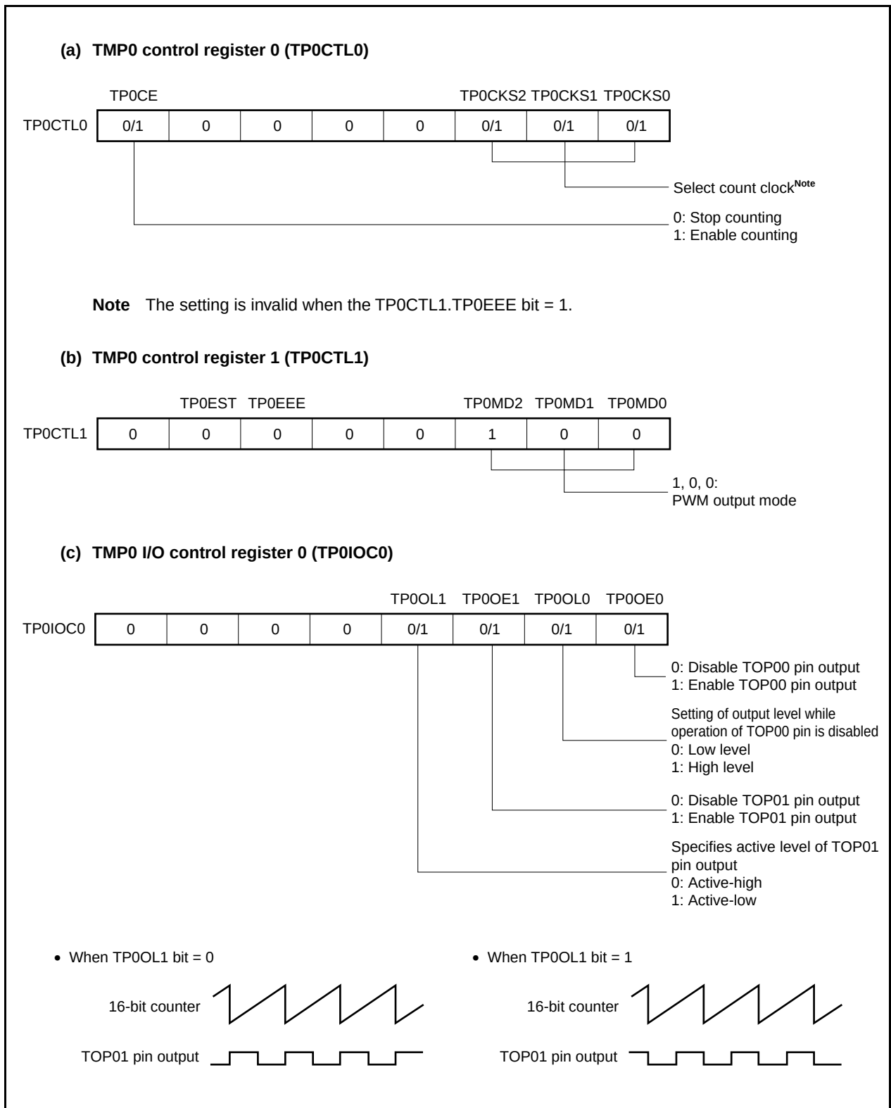
Figure 7-26. Register Setting in PWM Output Mode (1/2)
