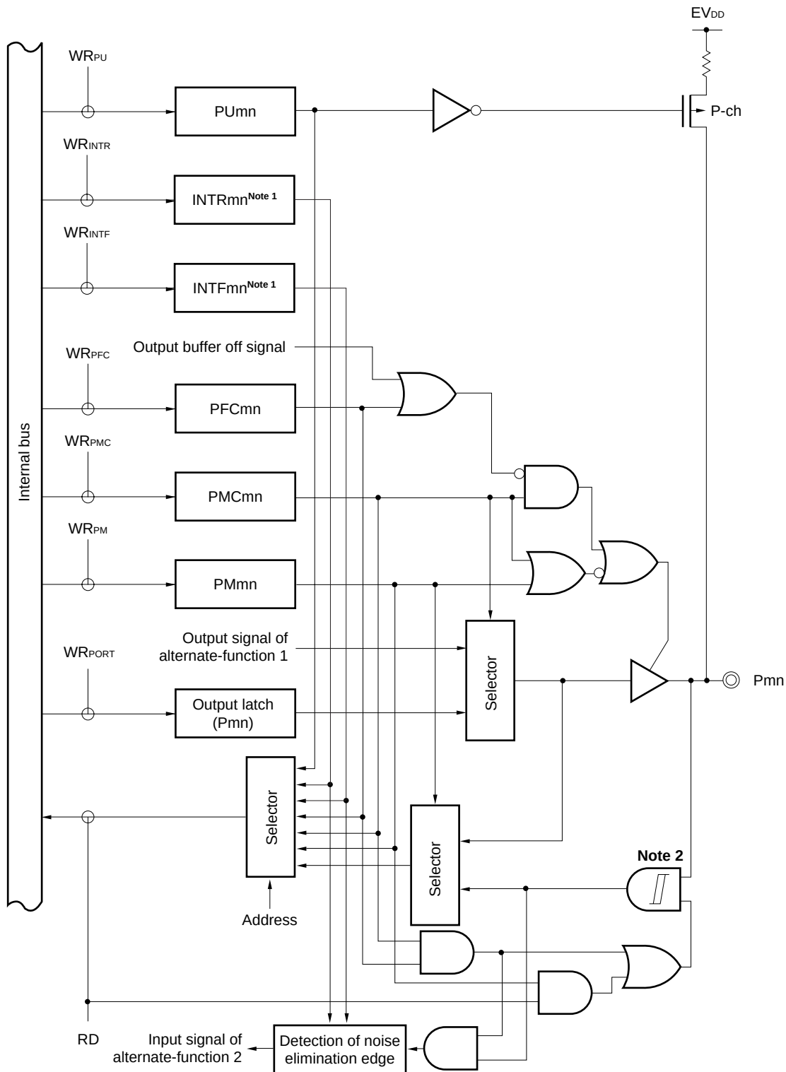
Figure 4-19. Block Diagram of Type E01-SUILZ
