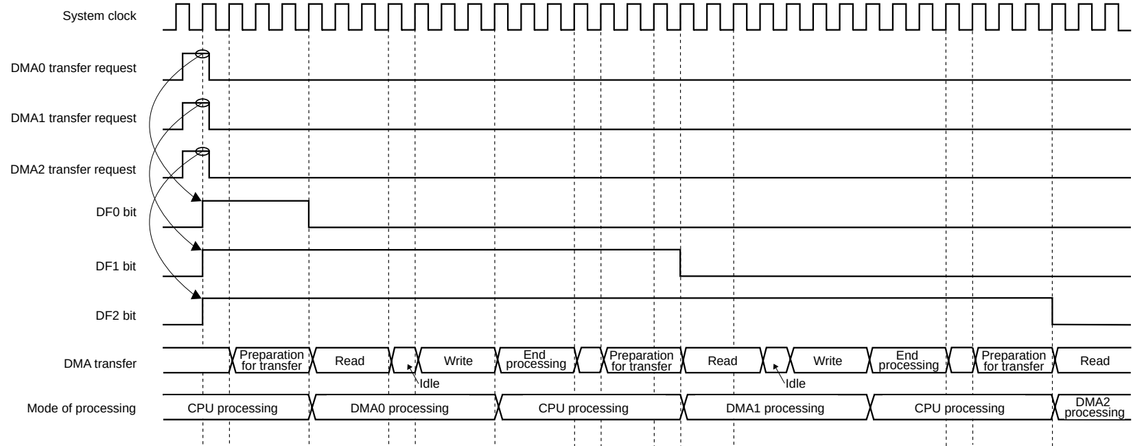
Figure 20-1. Priority of DMA (1)
