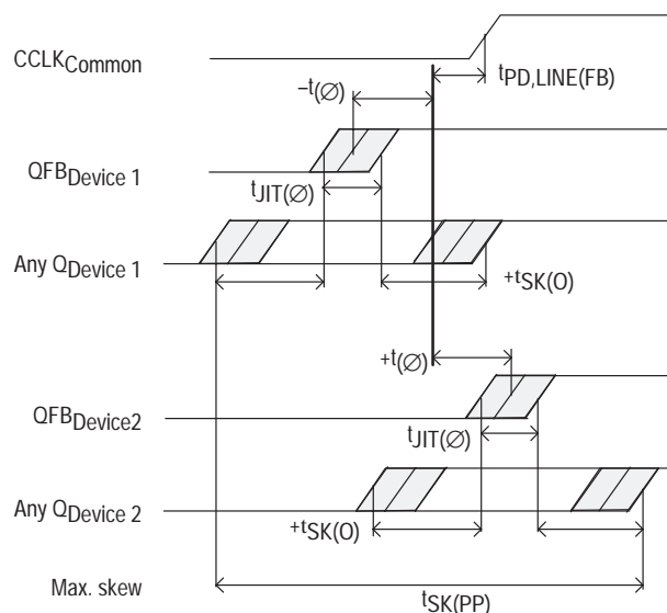
Figure 8. MPC97R72 max. device-to-device skew
