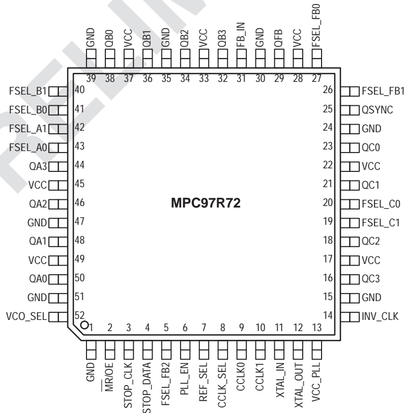
Figure 2. MPC97R72 52-Lead Package Pinout (Top View)
