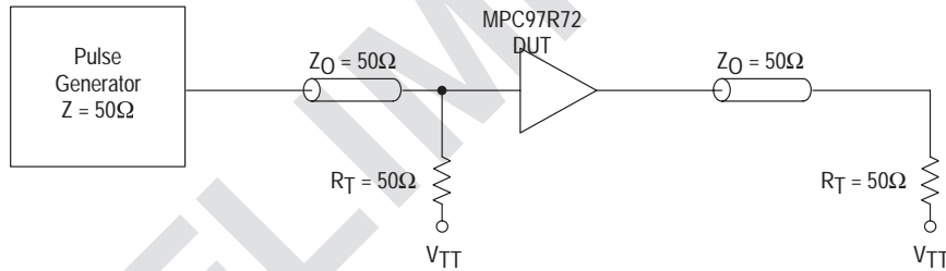
Figure 13. CCLK MPC97R72 AC test reference for V_{CC} = 3.3V and V_{CC} = 2.5V
