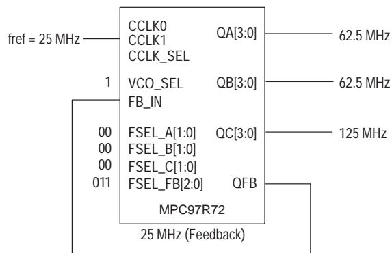
Figure 4. Example Configuration
