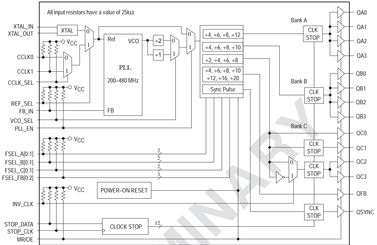
Figure 1. MPC97R72 Logic Diagram
