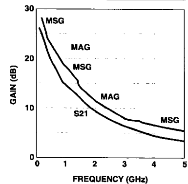
Figure 22. AT-31033 Gains vs. Frequency at V_{CE} = 2.7\text{ V} , I_C = 10\text{ mA} .
