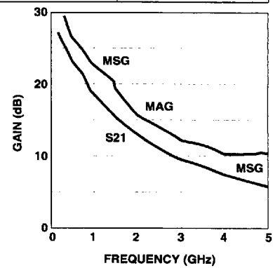
Figure 25. AT-31011 Gains vs. Frequency at V_{CE} = 5\text{ V} , I_C = 10\text{ mA} .
