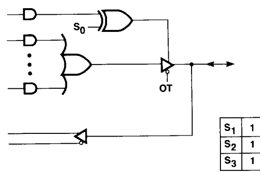
Figure 2h. I/O Feedback, Combinatorial Output, Active-HIGH Output
