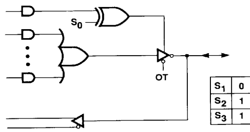
Figure 2d. I/O Feedback, Combinatorial Output, Active-LOW Output
