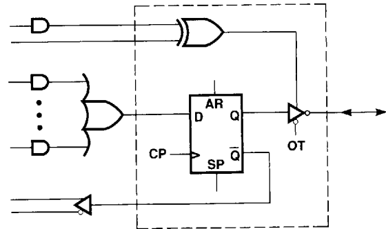
Figure 5. Buried register
