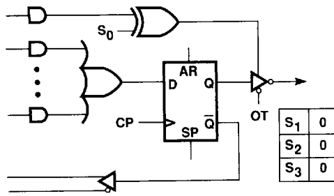
Figure 2a. Registered Feedback, Registered Output, Active-LOW Output
