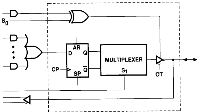
Figure 4. Output register
