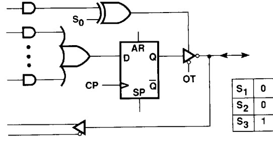
Figure 2b. I/O Feedback, Registered Output, Active-LOW Output
