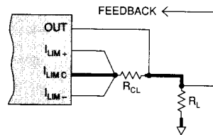
FIGURE 1. I_{LIMIT} WHERE I_{CL+} = I_{CL-}
