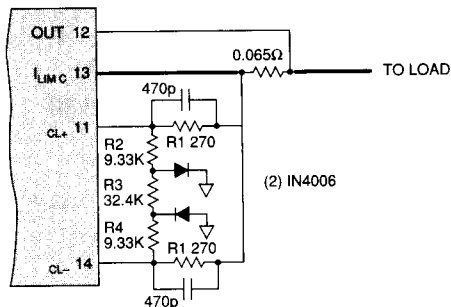
FIGURE 4. FOLDOVER CURRENT LIMIT
