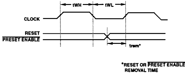
FIGURE 13. TIMING DIAGRAM DEFINING t_{rem}
