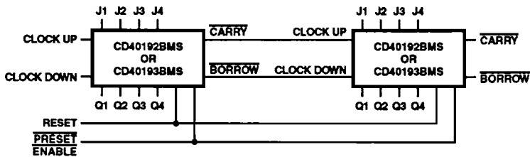
FIGURE 14. CASCADED COUNTER PACKAGES
