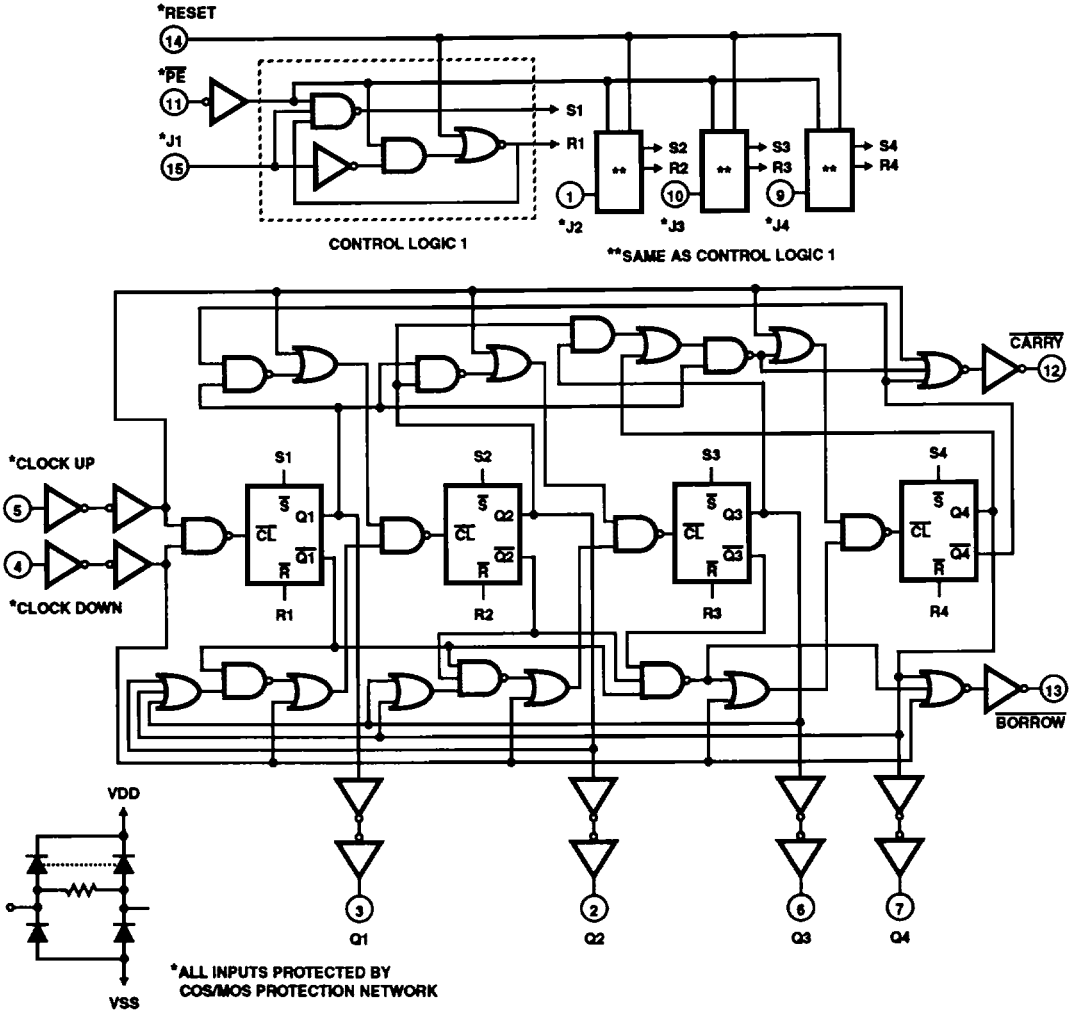
FIGURE 1. CD40192BMS LOGIC DIAGRAM (BCD)
