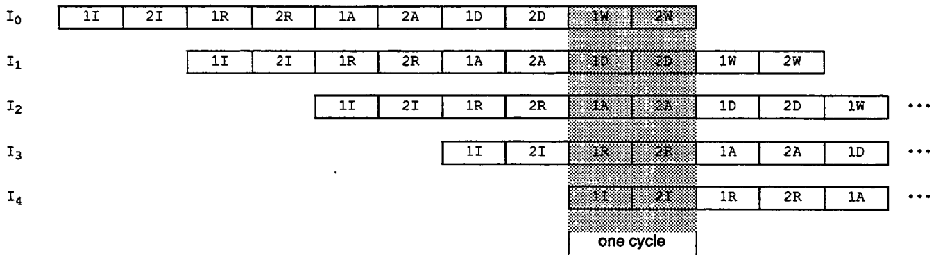
Figure 2. R4600 Pipeline
