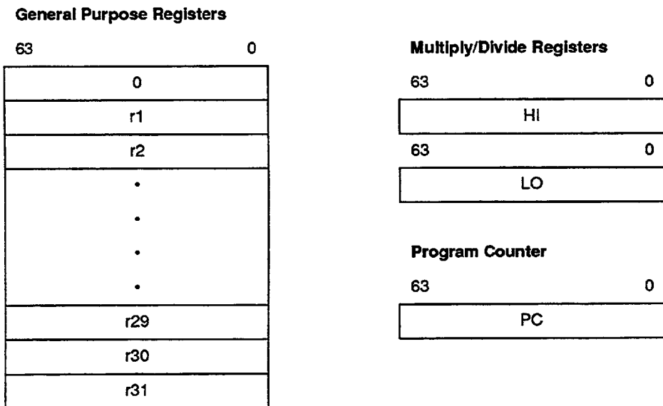
Figure 1. CPU Registers
