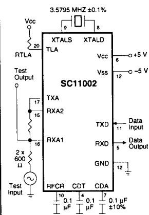
Figure 1. SC11002 AC Specification Circuit
