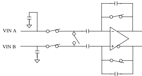
Figure 1 – Analog Input Equivalent Circuit
