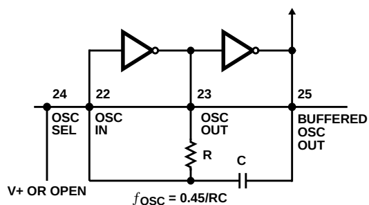
FIGURE 10. RC OSCILLATOR
