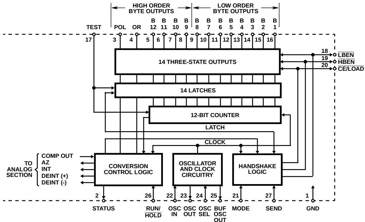
FIGURE 4. DIGITAL SECTION
