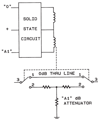
Figure 1. Cell Schematic
