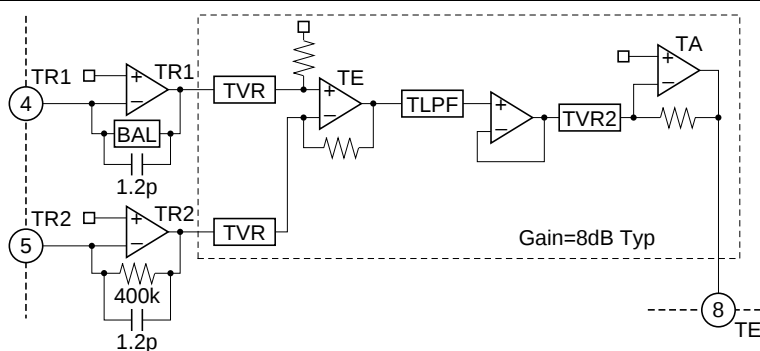
Figure 12 Tracking Error Amplifiers
