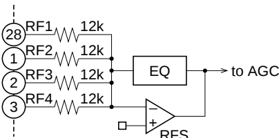
Figure 3 RFS Amplifier
