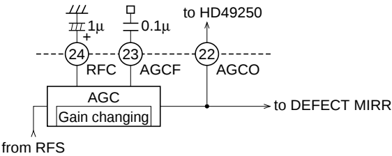
Figure 5 AGC Amplifier
