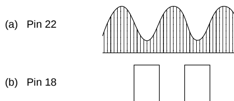
Figure 11 Mirror Detection Waveform
