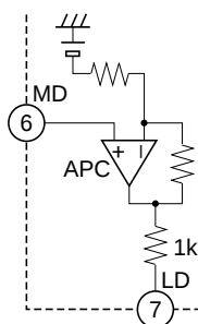
Figure 7 APC
