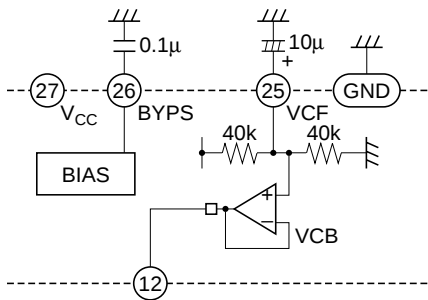
Figure 13 Bias, Reference Voltage
