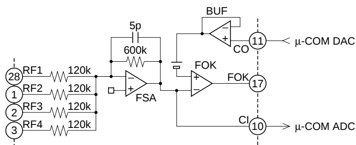
Figure 6 FOK Detection
