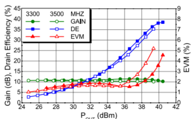
Figure 5 - OFDM Performance Tuned for P_{OUT} at 2% EVM in Load-Pull System
