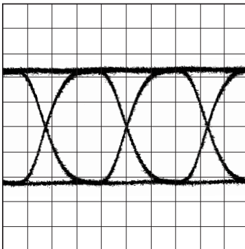
NRZ Transmit Output (TX±)
