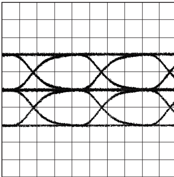
A 0 Meter UTP-5 Cable 500mV/DIV, 2ns/DIV
