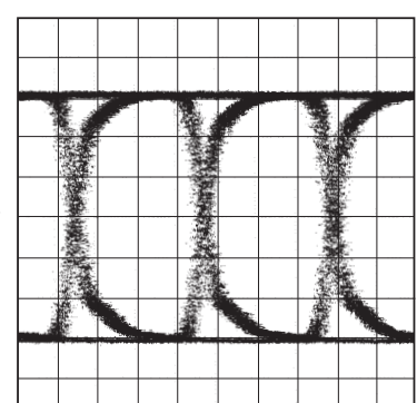
NRZ Receiver Output (RD±)
