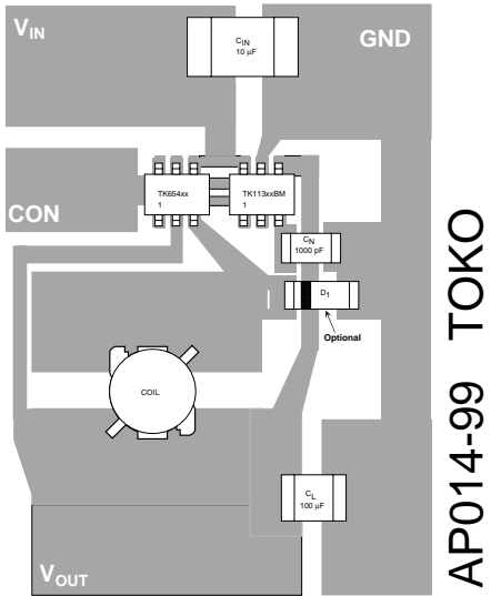
FIGURE 14: BUCK AND LINEAR APPLICATION BOARD LAYOUT
