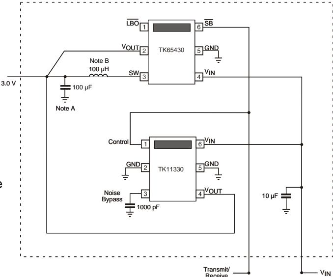
FIGURE 13: BUCK AND LINEAR SCHEMATIC
