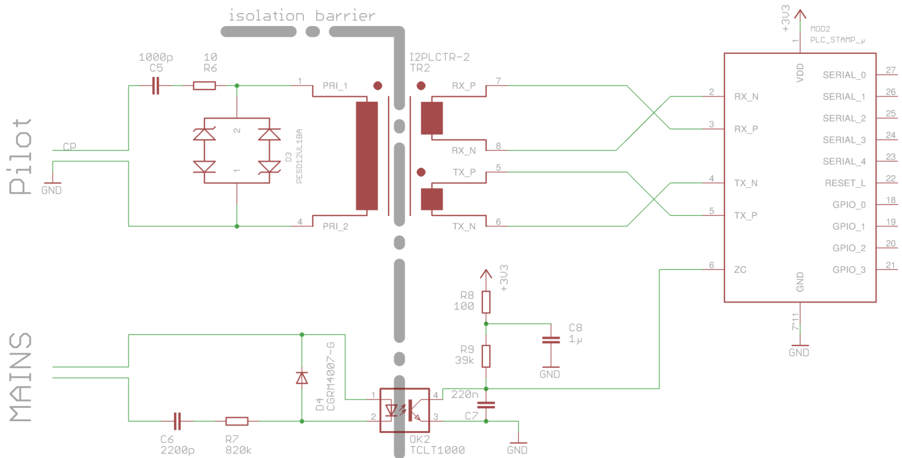
Figure 7 Reference Schematics for PLC Coupling to the Pilot Signal
