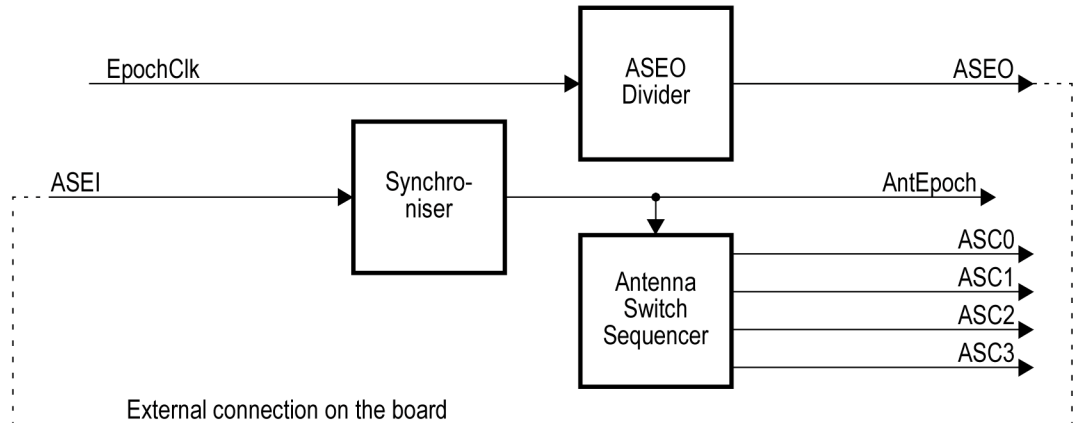
Figure 22. Antenna Switch Controller block diagram
