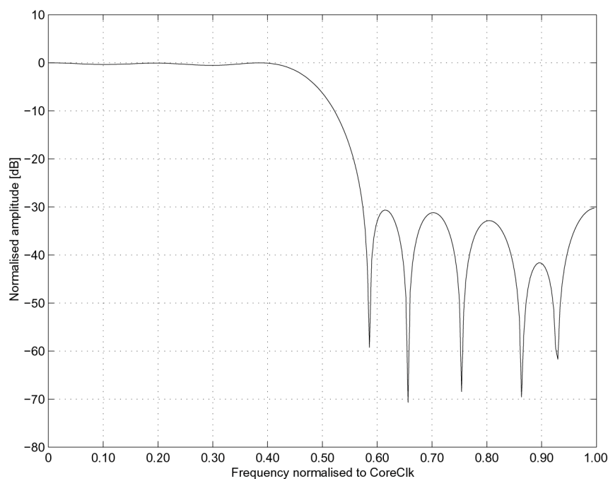
Figure 4. Overall Filter response for the Lowpass Filter
