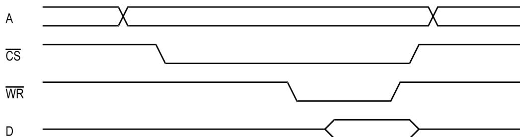
Figure 26. Example write access to the AGGA-2
