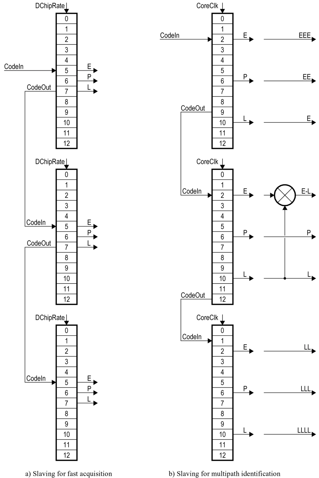
Figure 16. Two examples of three channels with slaved Code Delay Lines
