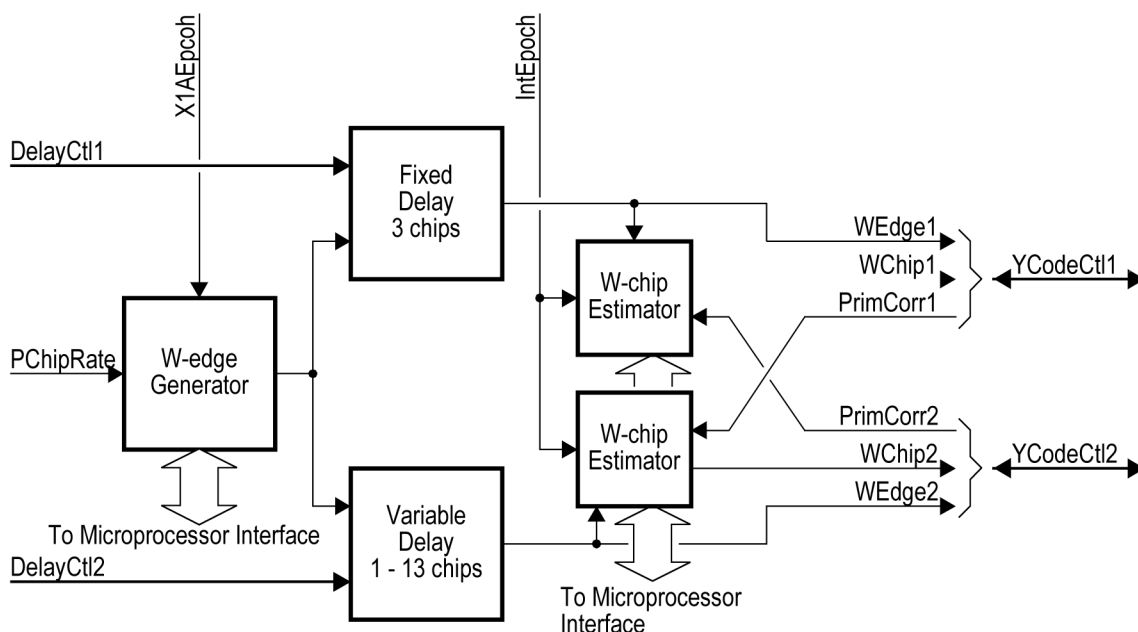
Figure 20. Semi-codeless Controller block diagram
