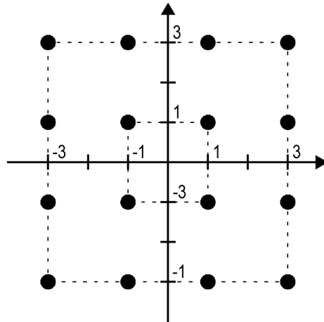
Figure 12. Complex signal constellation
