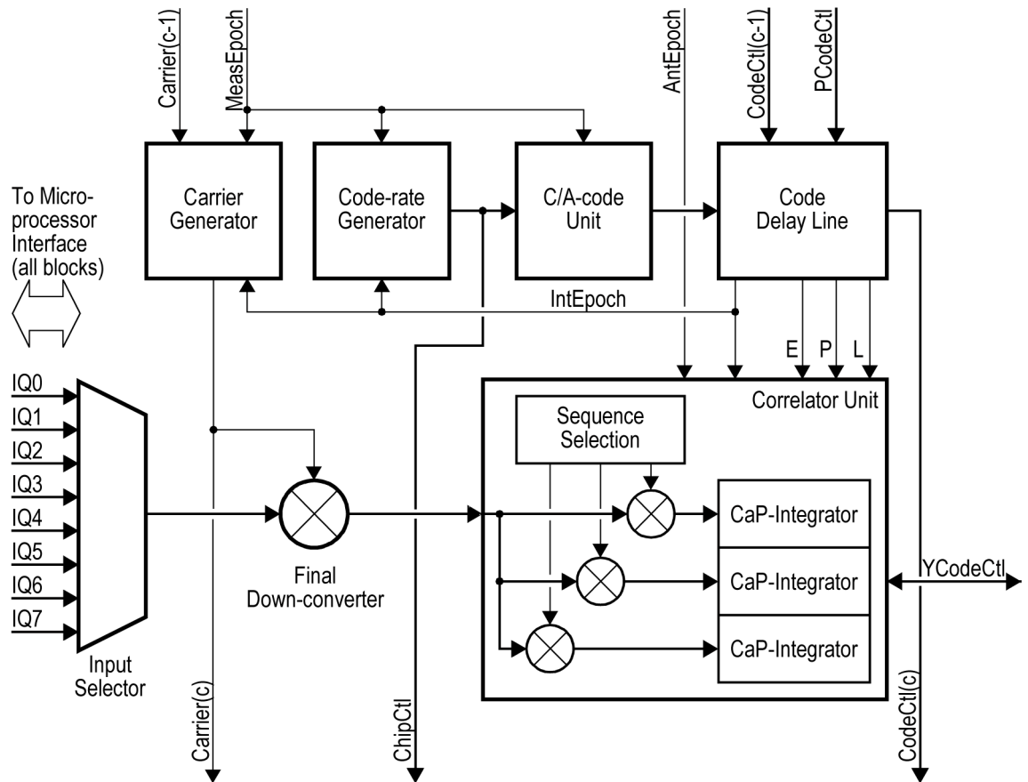
Figure 7. CaP-channel block diagram
