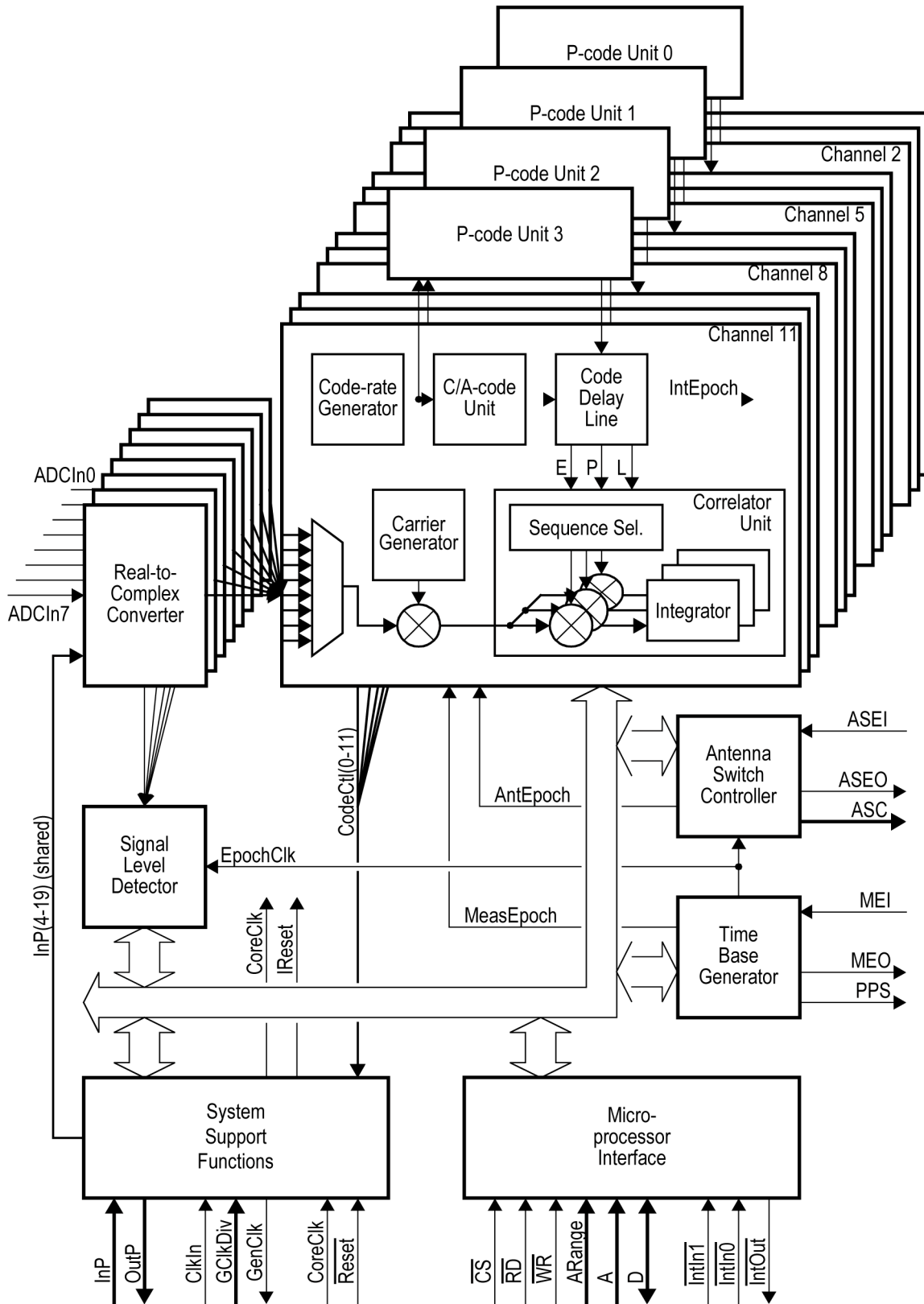
Figure 1. AGGA-2 block diagram
