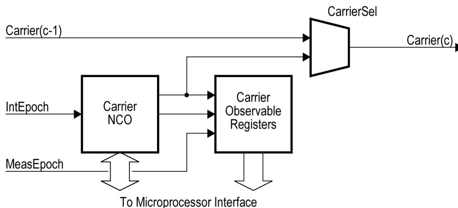
Figure 11. Carrier Generator block diagram
