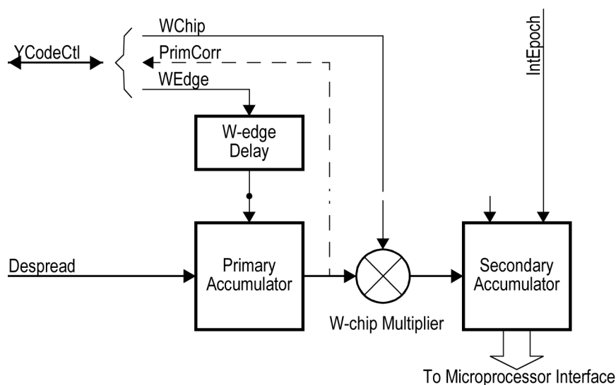
Figure 18. CaP-Integrator configured for semi-codeless operation
