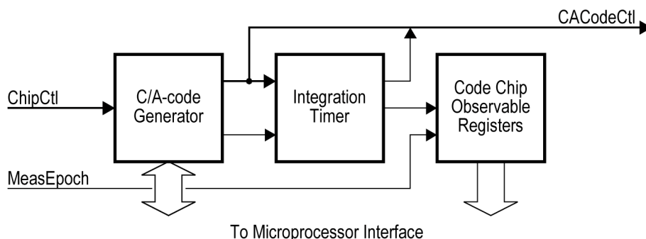
Figure 14. C/A-code Unit block diagram
