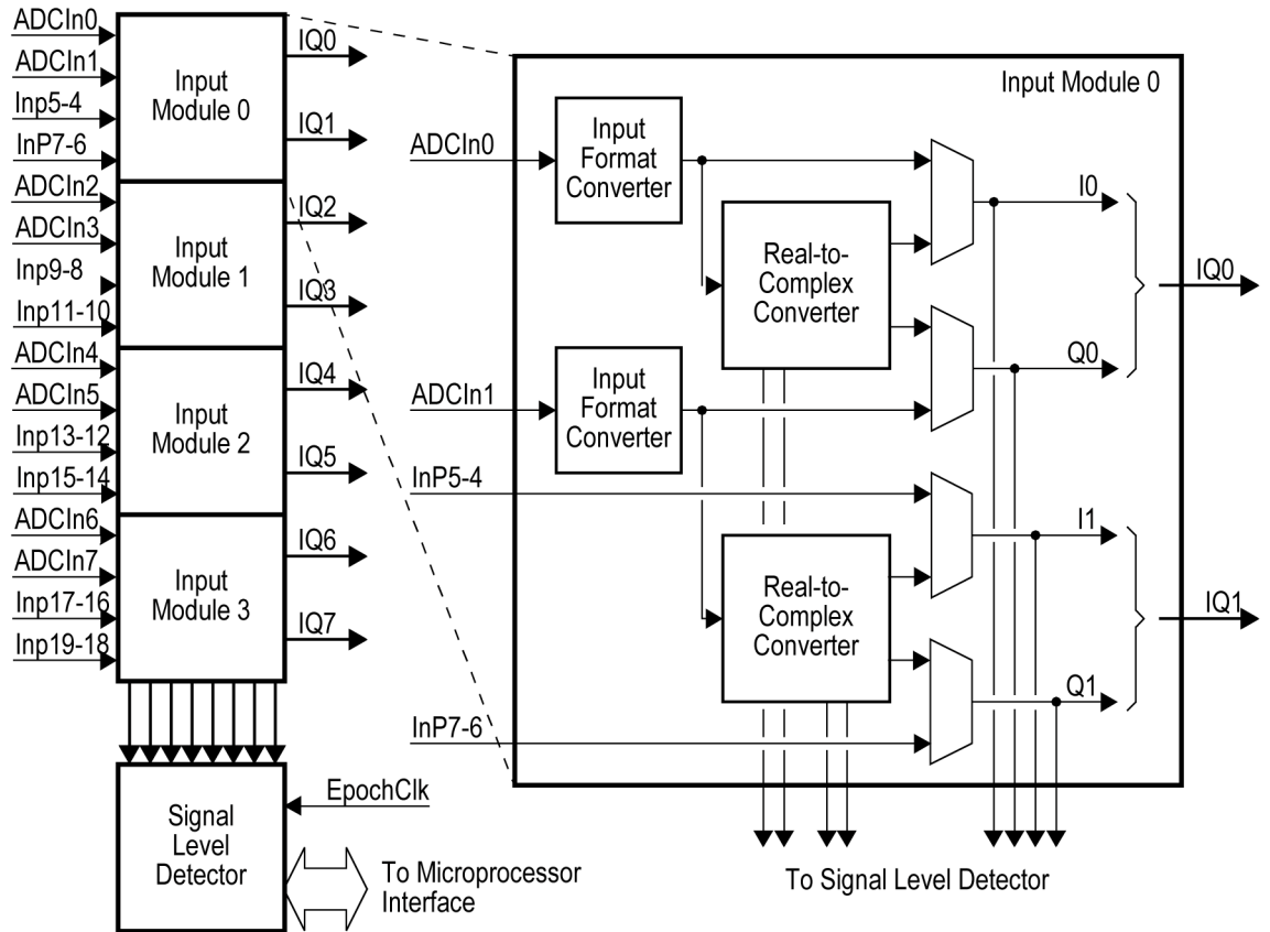
Figure 2. Front-end Interface block diagram
