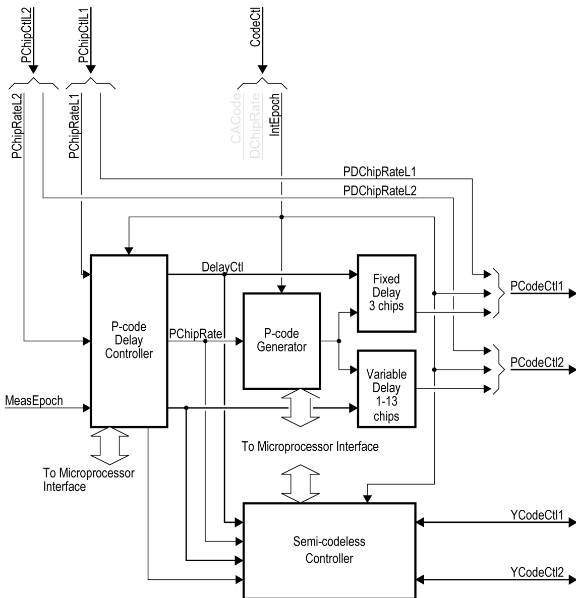
Figure 19. P-code Unit block diagram
