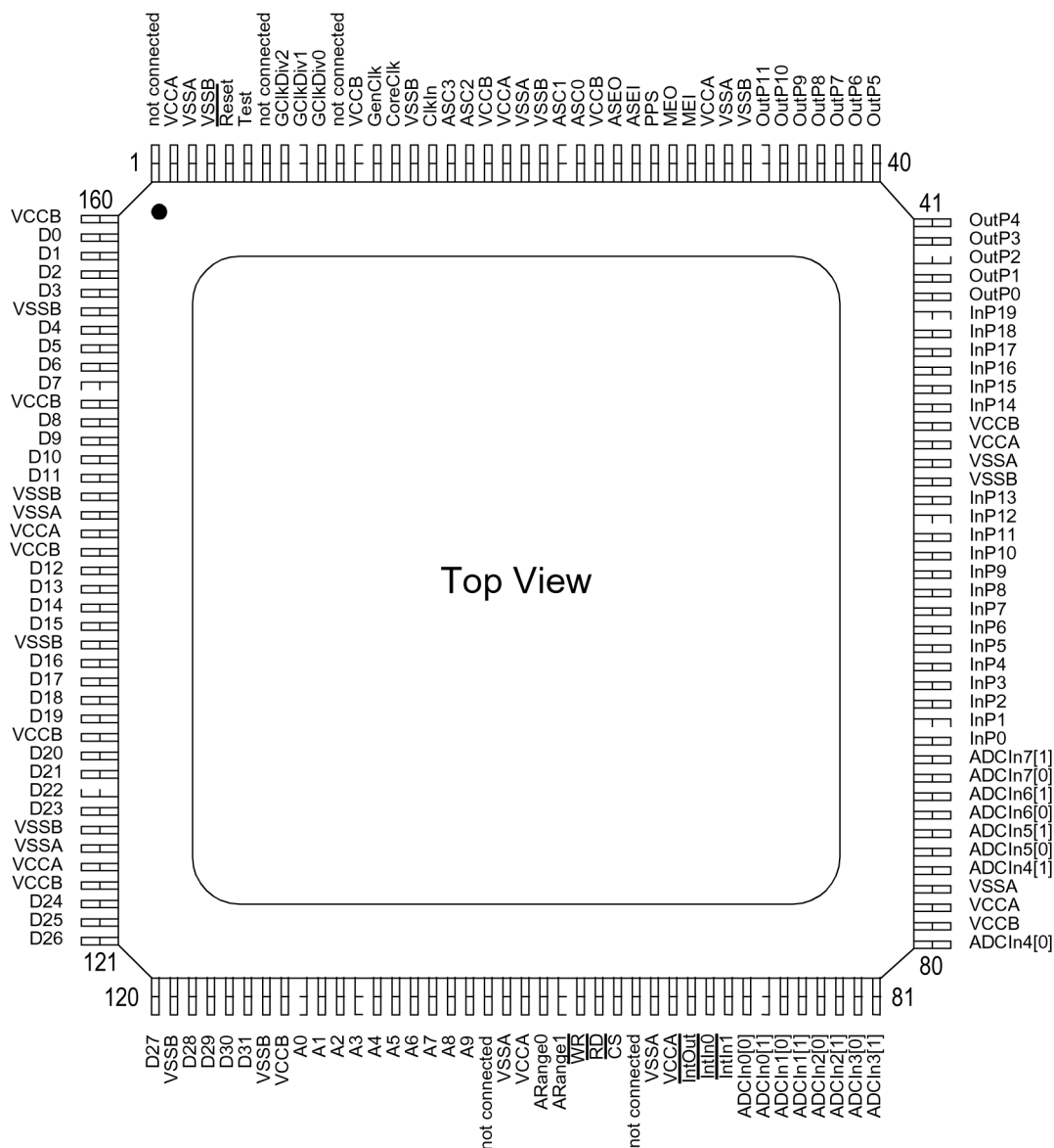
Figure 28. AGGA 2 pinout
