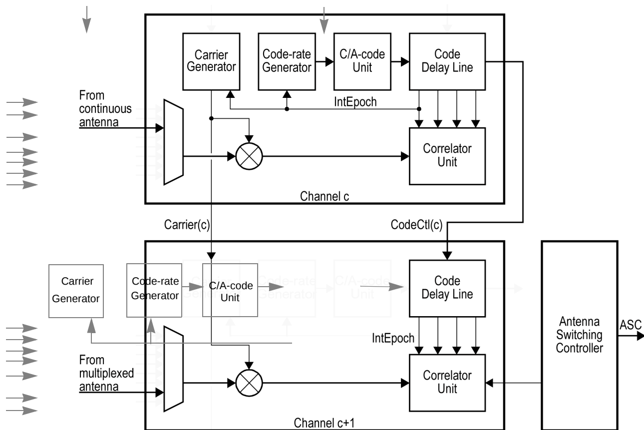
Figure 8. Two channels slaved for Hybrid Parallel Multiplex attitude determination
