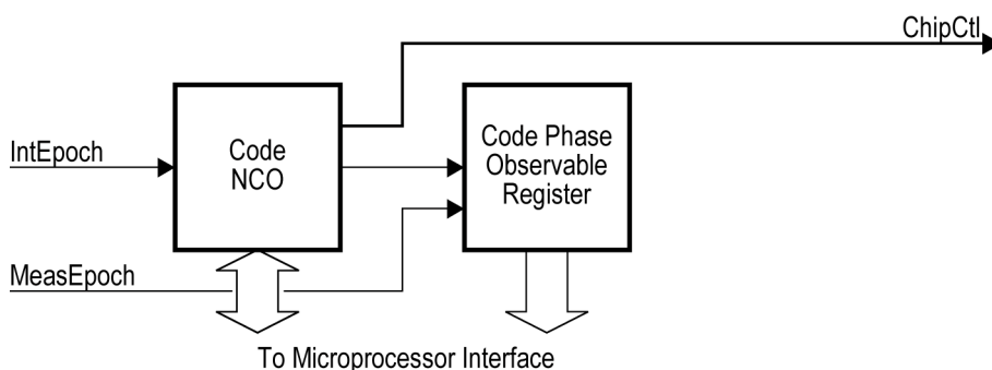
Figure 13. Code-rate Generator block diagram
