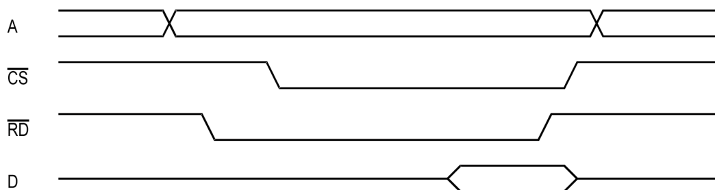
Figure 25. Example Read Access to the AGGA-2
