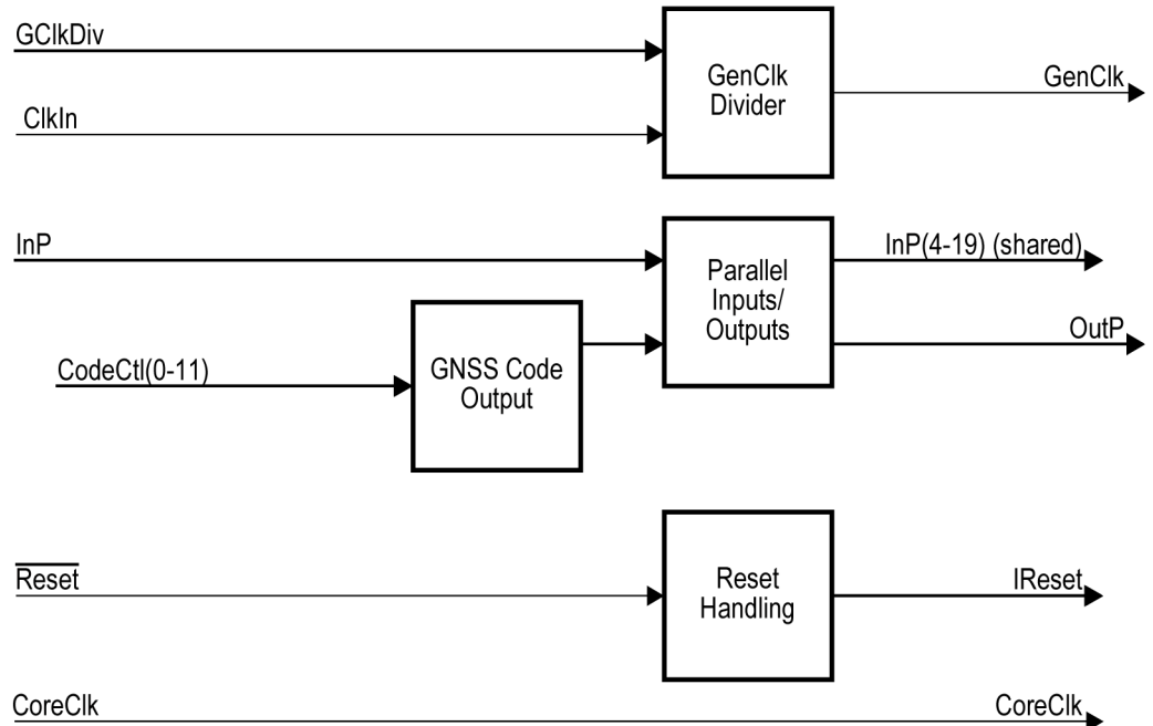
Figure 23. System Support Functions block diagram
