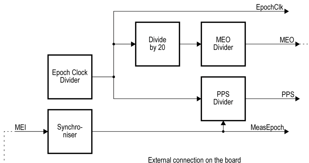
Figure 21. Time Base Generator block diagram
