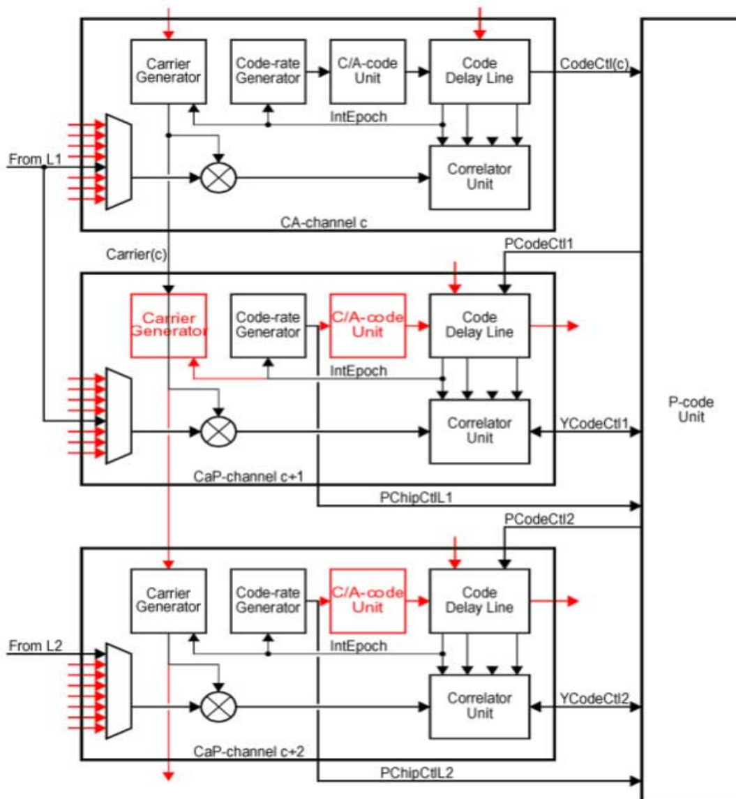
Figure 10. Three channels slaved for dual frequency operation
