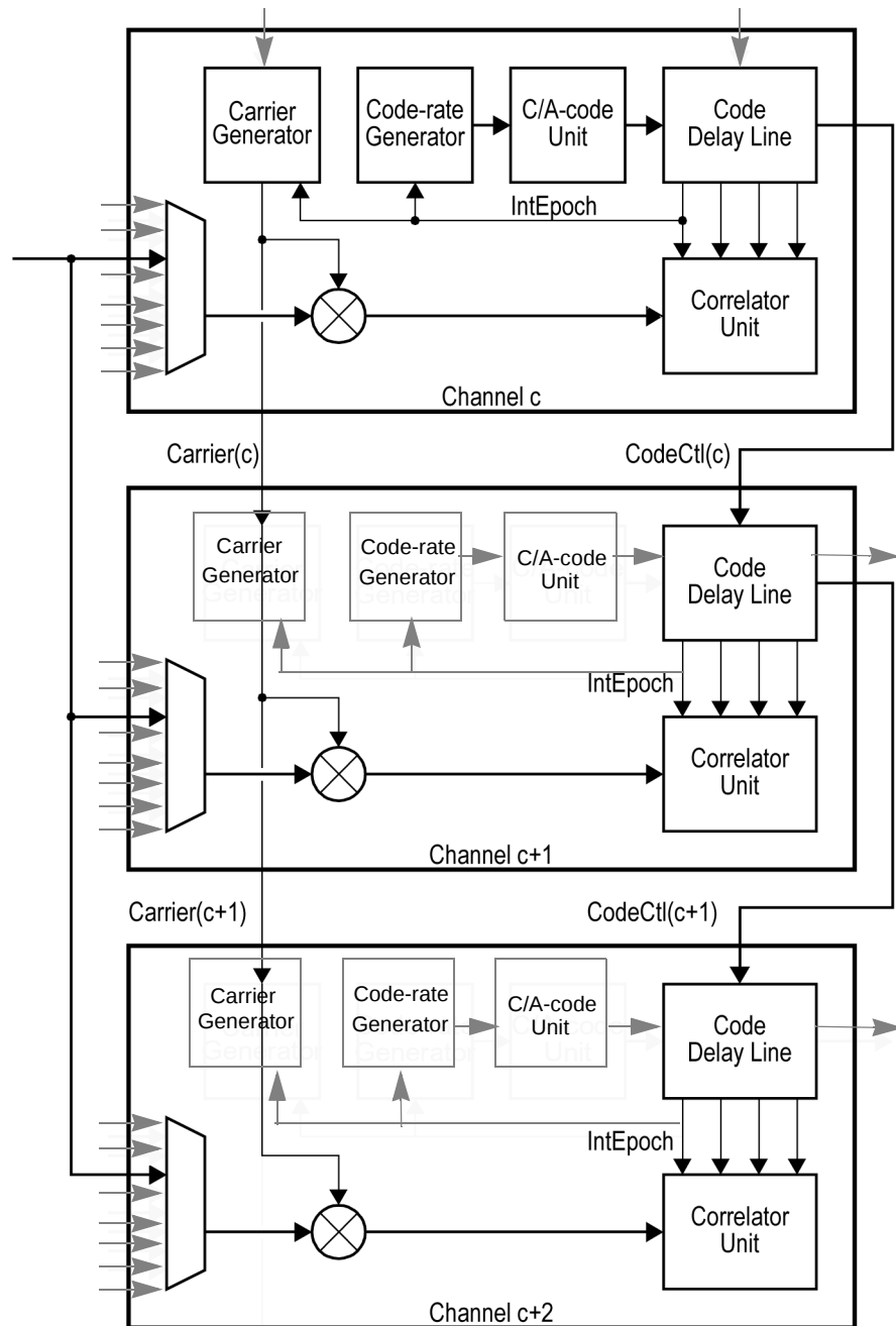
Figure 9. Three channels slaved for fast acquisition or multipath identification
