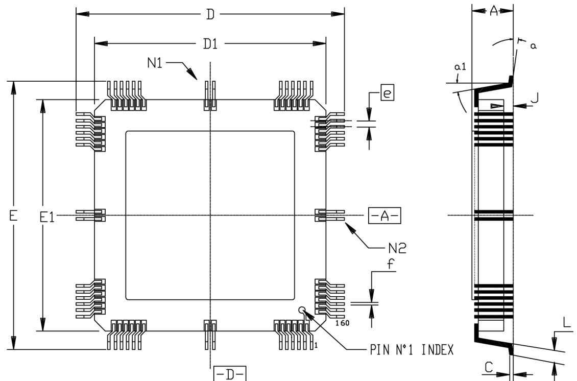
Figure 27. AGGA 2 mechanical data
