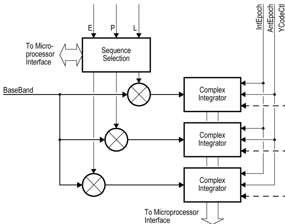
Figure 17. Correlator Unit block diagram
