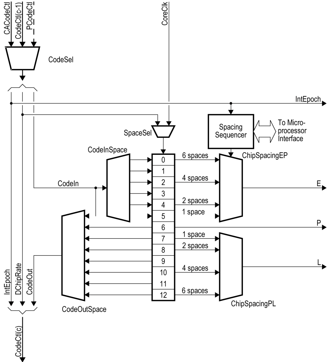
Figure 15. Code Delay Line block diagram
