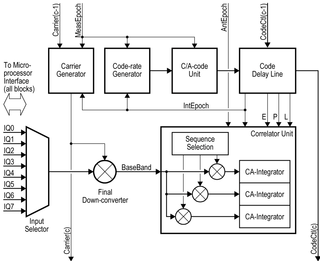
Figure 6. CA-channel block diagram
