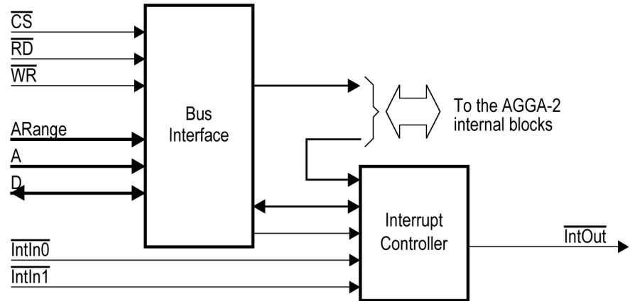
Figure 24. Microprocessor Interface block diagram
