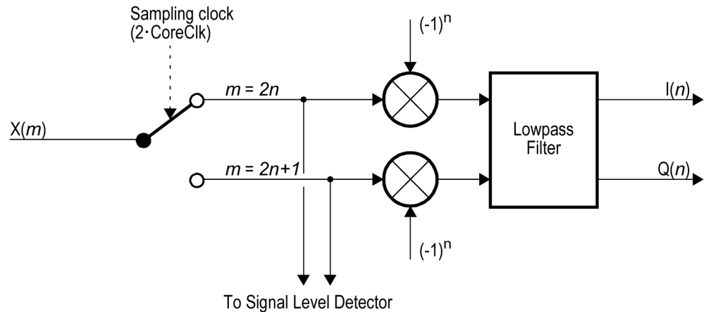
Figure 3. Real-to-Complex Converter block diagram
