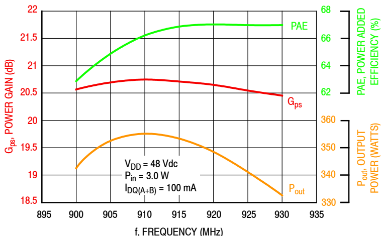
Figure 6. Power Gain, Power Added Efficiency and Output Power versus Frequency at a Constant Input Power
